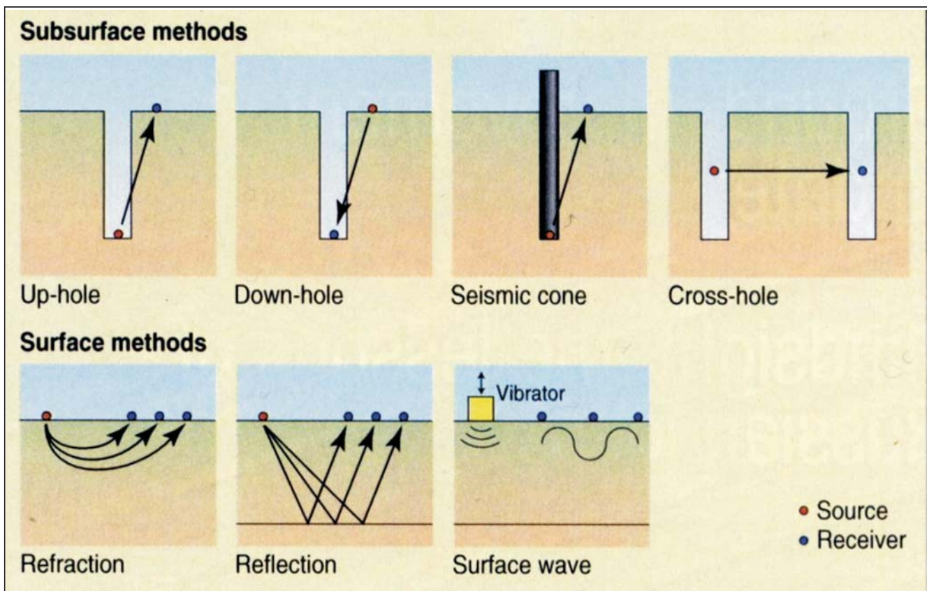
Fig. 6. Different types of subsurface and surface methods for hardness determining
