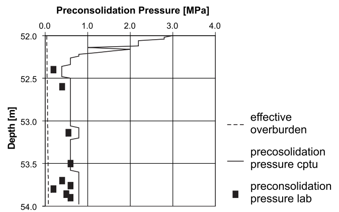
Fig. 13. Clay from the Belchatów Mine, test CPTU B9602, interpretation of friction angle
