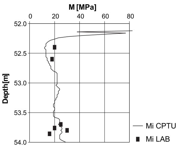
Fig. 11. Clay from the Belchatów Mine, test CPTU B9602, interpretation of preconsolidation pressure
