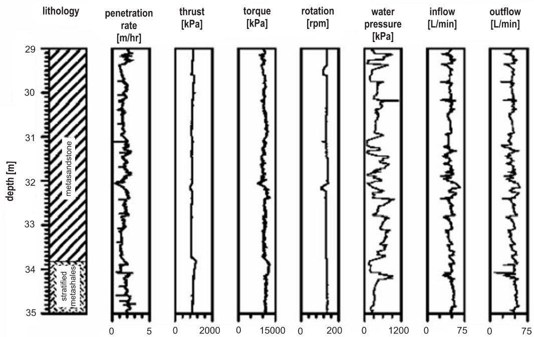
Fig. 3. Results of MDW — monitoring in a drilled hole
