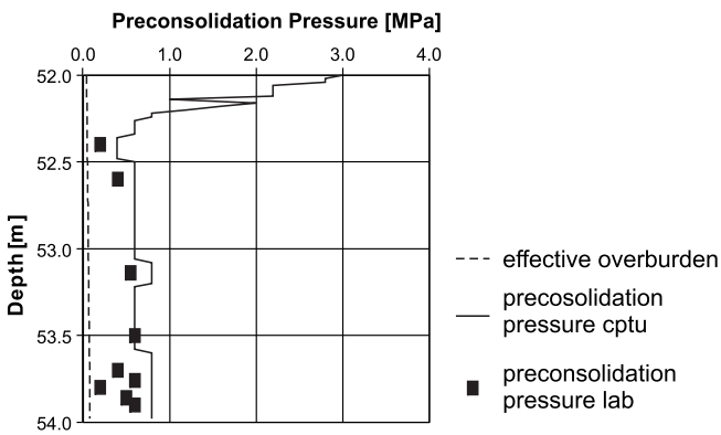
Fig. 10. Clay from Belchatów Mine, test CPTU B9602, interpretation of the preconsolidation pressure
