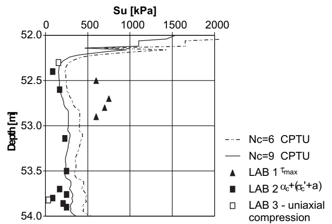
Fig. 12. Clay from the Belchatów Mine, test CPTU B9602, undrained shear strength interpretation Su (correlation factor Nc = 6–9)
