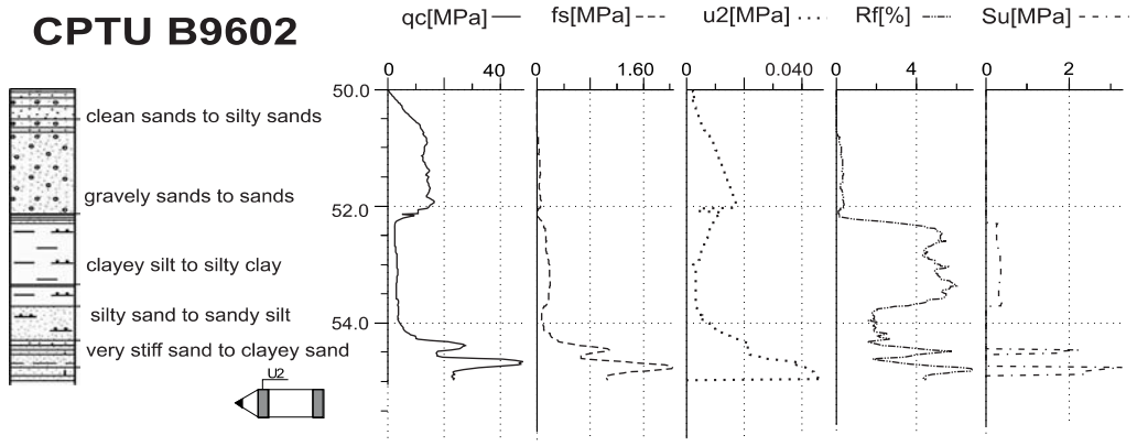
Fig. 9. CPTU test performed by author in near to a landslide on the southern slope of the Belchatów open-pit mine 50 m below the natural terrain level
