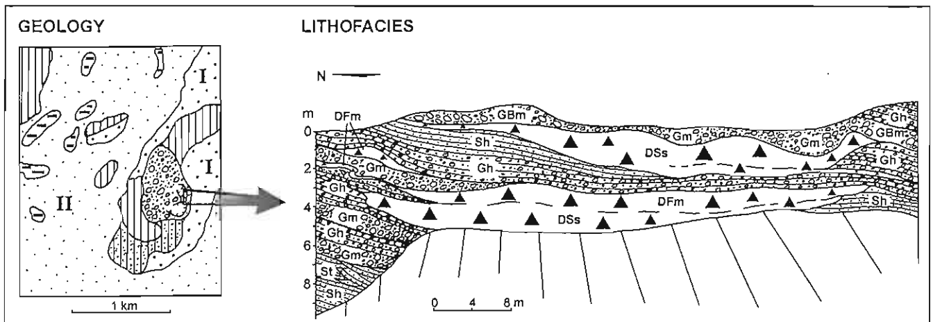
Fig. 7. Depositional end moraine at the maximum ice sheet limit of the Vistulian Glaciation to the south-east of Koszelewy
