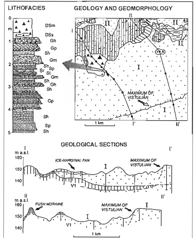
Fig. 4. Ice-marginal features at the ice sheet maximum limit of the Vistulian Glaciation to the south of Lidzbark Welski
