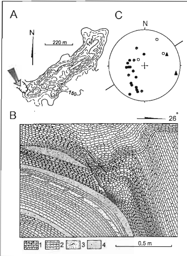
Fig. 5. Push moraine to the south of Lidzbark Welski
