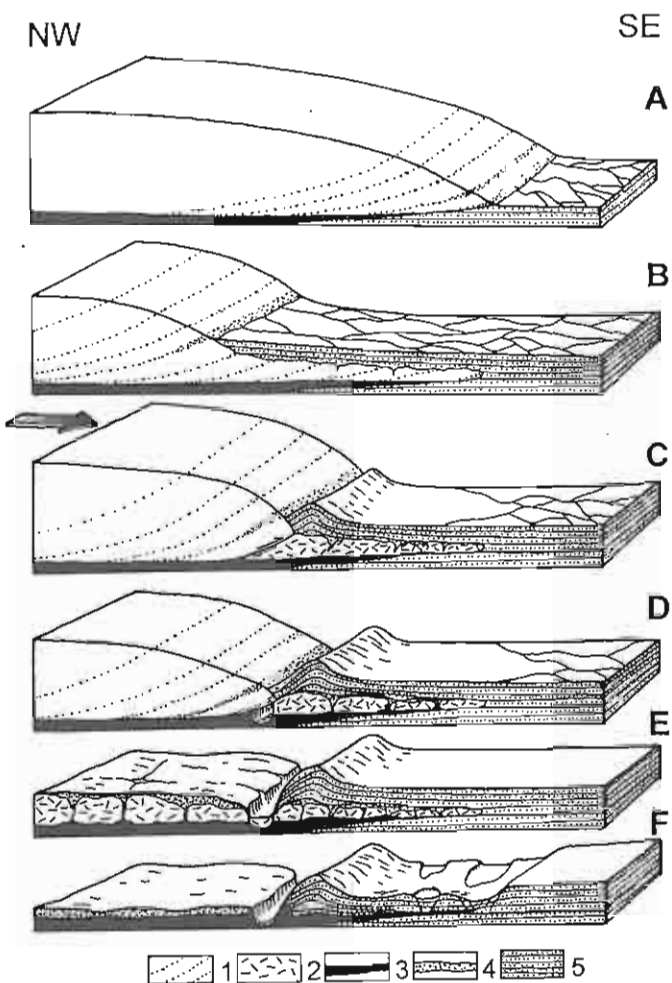
Fig. 6. The model of development of ice-marginal features during a maximum ice sheet limit of the Vistulian Glaciation to the south of Lidzbark Welski (explanations in the text)
