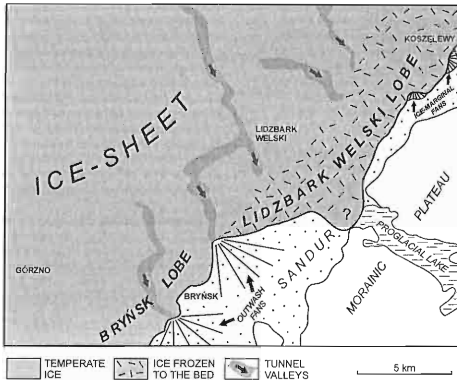
Fig. 8. Ice sheet dynamics during the maximum limit of the Vistulian Glaciation in the mid-eastern Chełmno–Dobrzyń Lakeland
