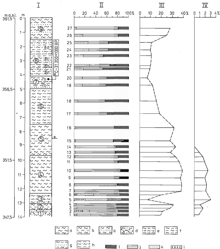
Fig. 4. Lithologic profile of the drilling Harbutowice-1 with results of grain size distribution
