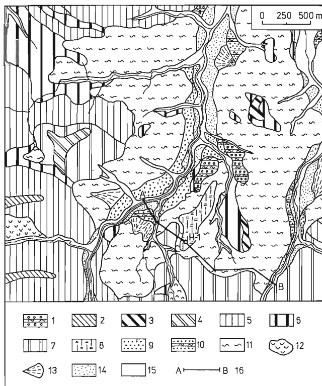
Fig. 2. Geologic map of the Quaternary deposits in the study area
