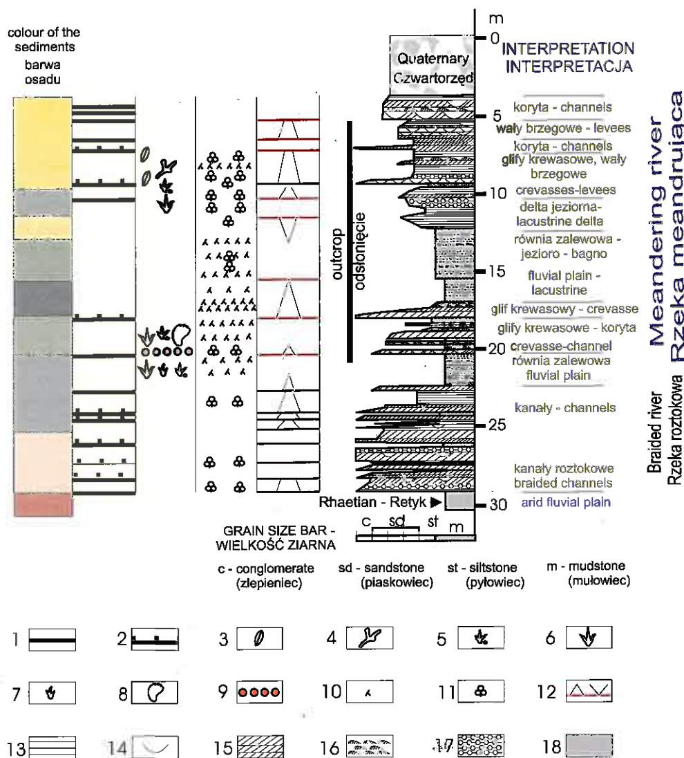
Fig. 2. Section of the Sołtyków borehole (section exposed in the outcrop is marked by the bar) and sedimentological interpretation
