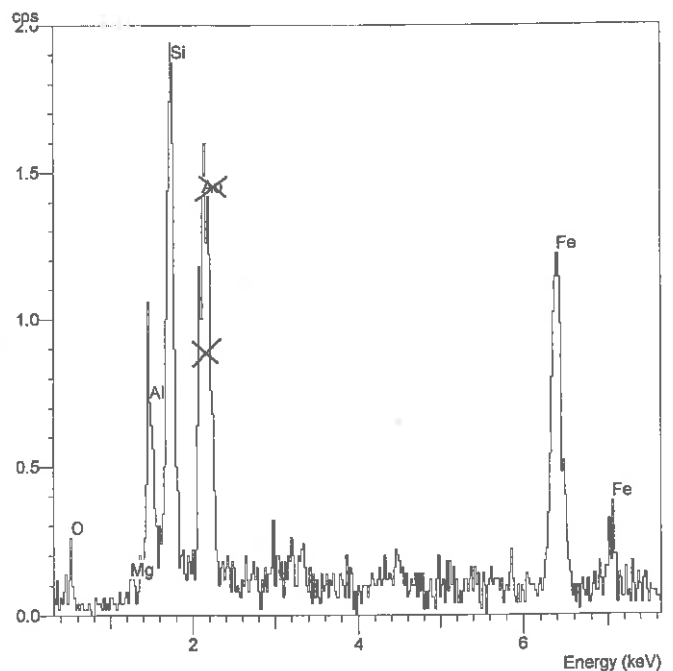
Fig. 5. Elements present in the infilling of the egg structures (EDS). Typical picture of illite mixed with iron hydroxides/oxides and some silica
