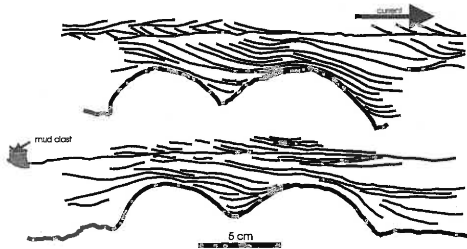
Fig. 4. Cross-section of the nest showing the cross-bedding in the sediment covering the egg structures. Note the concordant arrangement of the cross laminae, proving that the structures were present before the deposition of the host sediment
