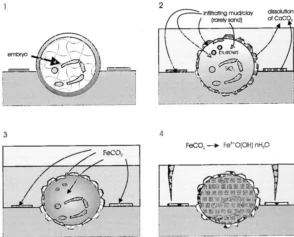
Fig. 11. Scheme showing stages of taphonomy and diagenesis of the post-egg structures
