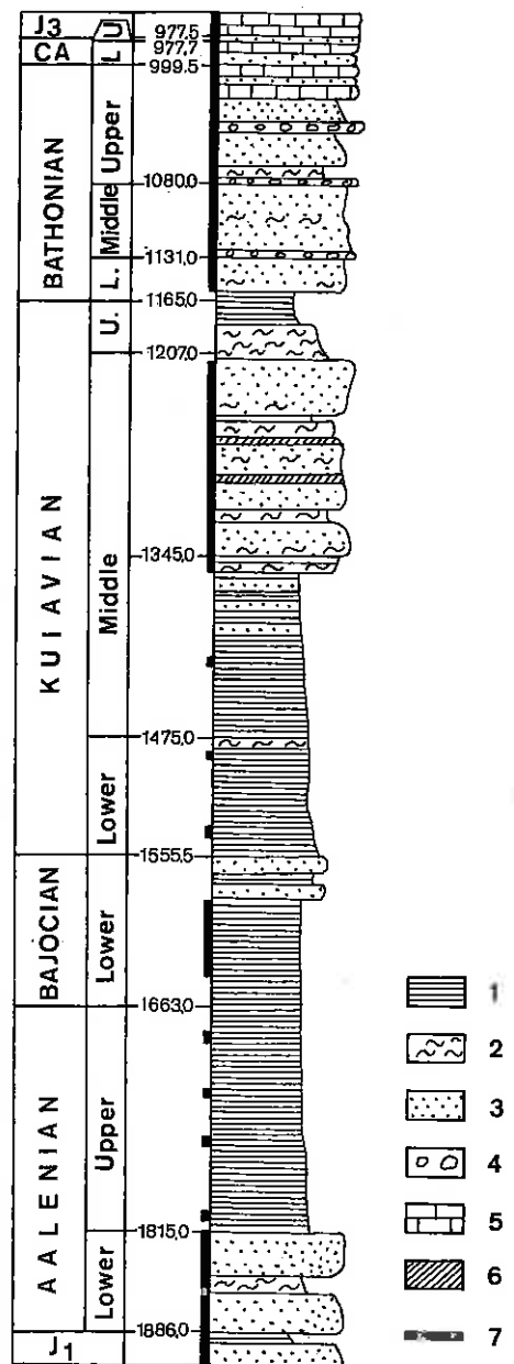
Fig. 2. Simplified lithological-stratigraphical section of the Middle Jurassic deposits from the borehole Wojszyce IG 4 (after A. Feldman-Olszewska, 1997)
