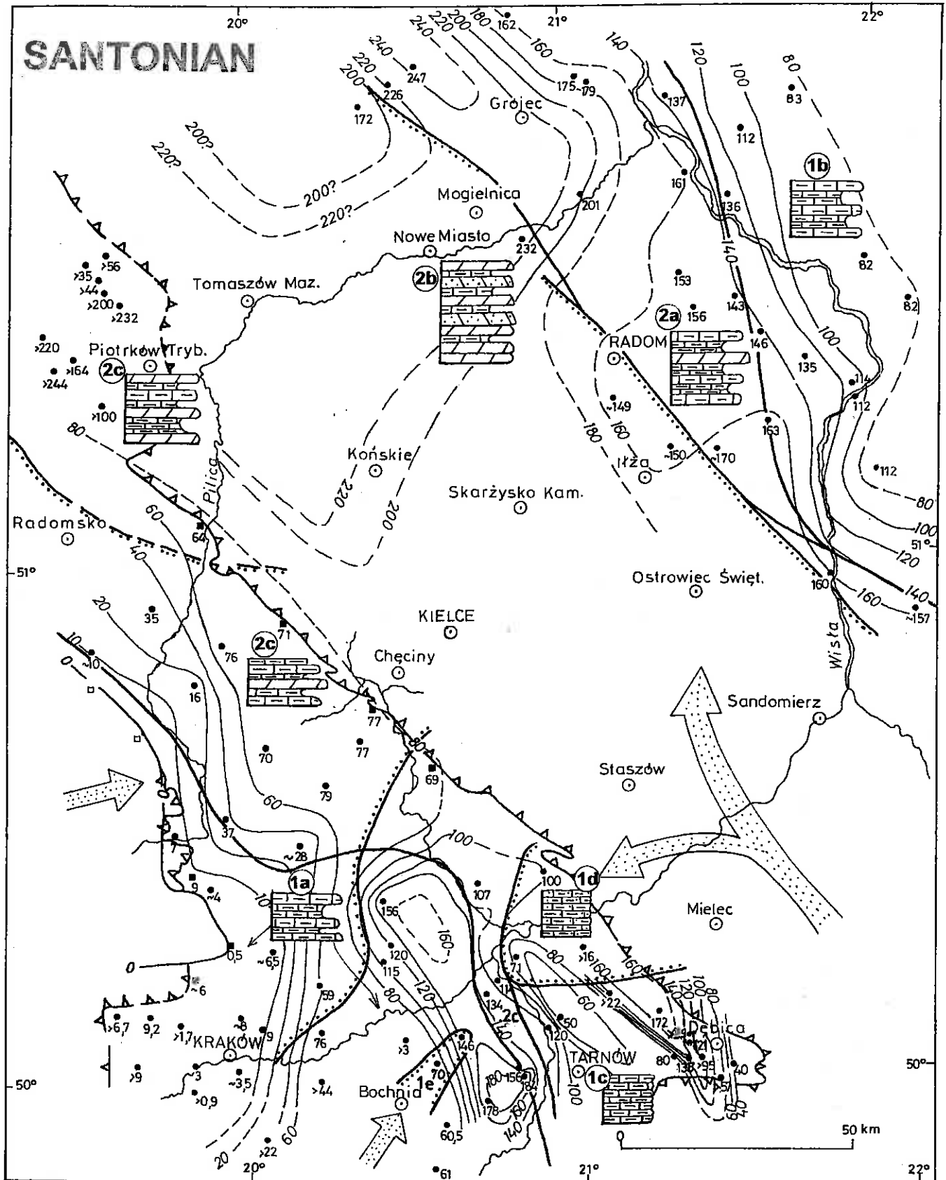
Fig. 8. Thickness and facies patterns of Santonian deposits Explanations see Figs. 1, 2 and 4
