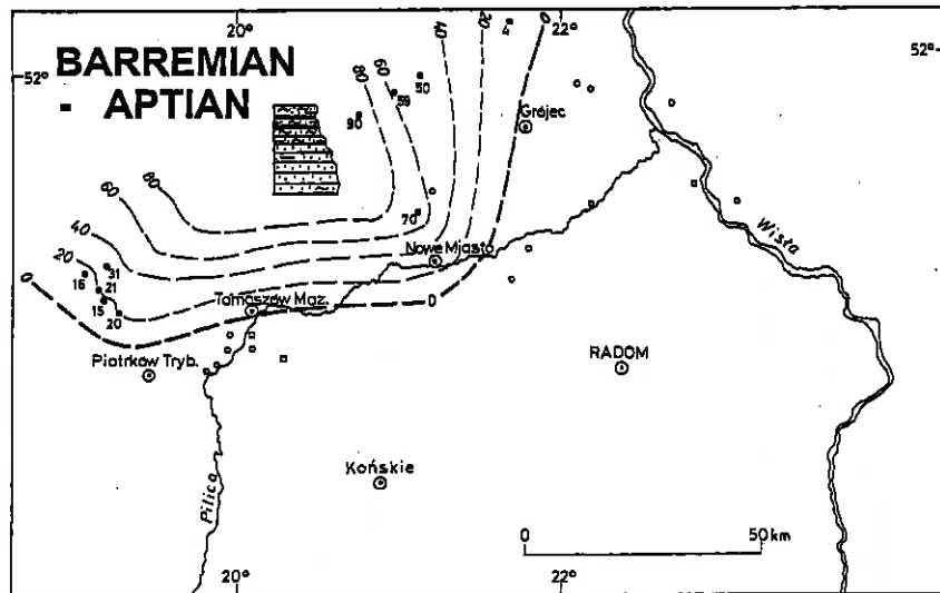
Fig. 3. Thickness and facies patterns of Barremian and Aptian deposits Explanations see Figs. 1 and 2
