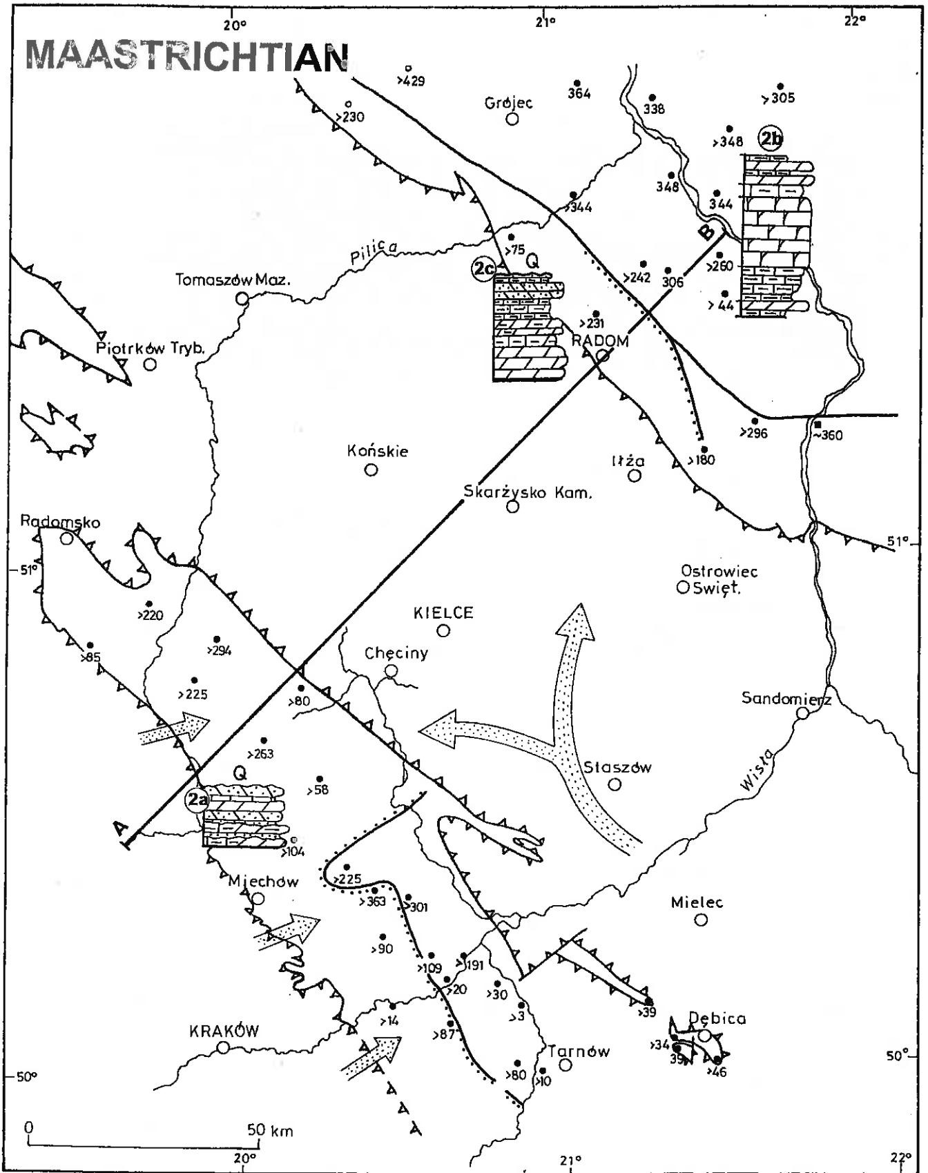
Fig. 10. Thickness and facies patterns of Maastrichtian deposits
