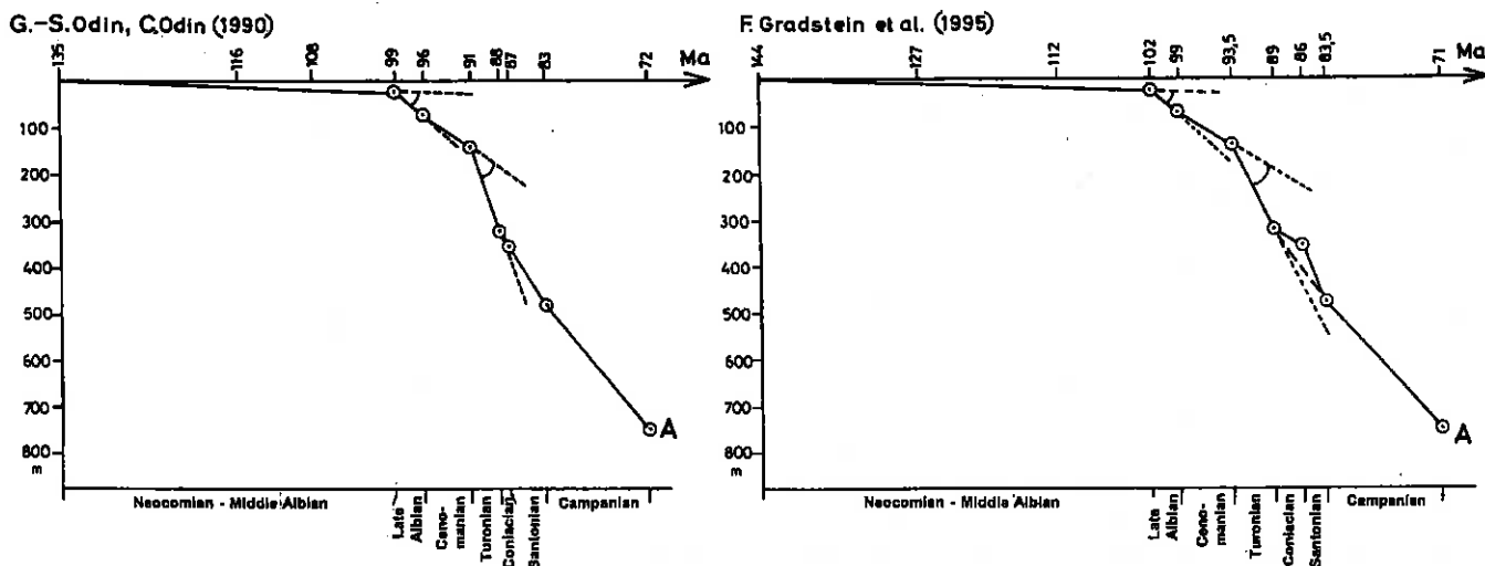
Fig. 13. Curve of medium subsidence along the cross-section Pilica-Radom-Kozienice Location on Fig. 10
