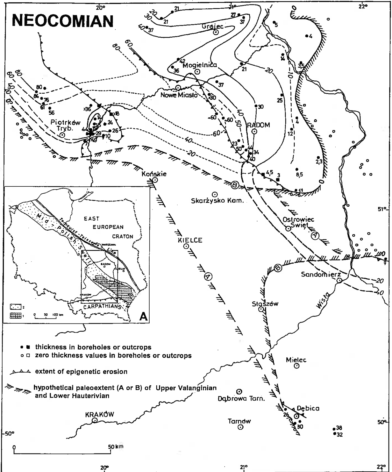
Fig. 1. Thickness pattern of Neocomian deposits (A — location of investigated area)
