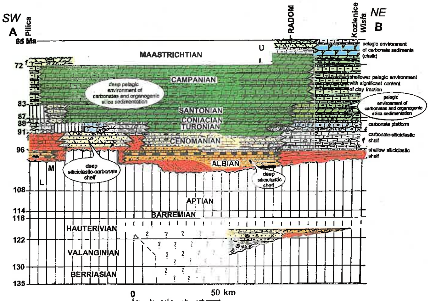
Fig. 11. Chronostratigraphic diagram of lithofacies and sedimentary environments characteristic for Holy Cross segment of the Mid-Polish Trough Lithological explanations see Figs. 2 and 4
