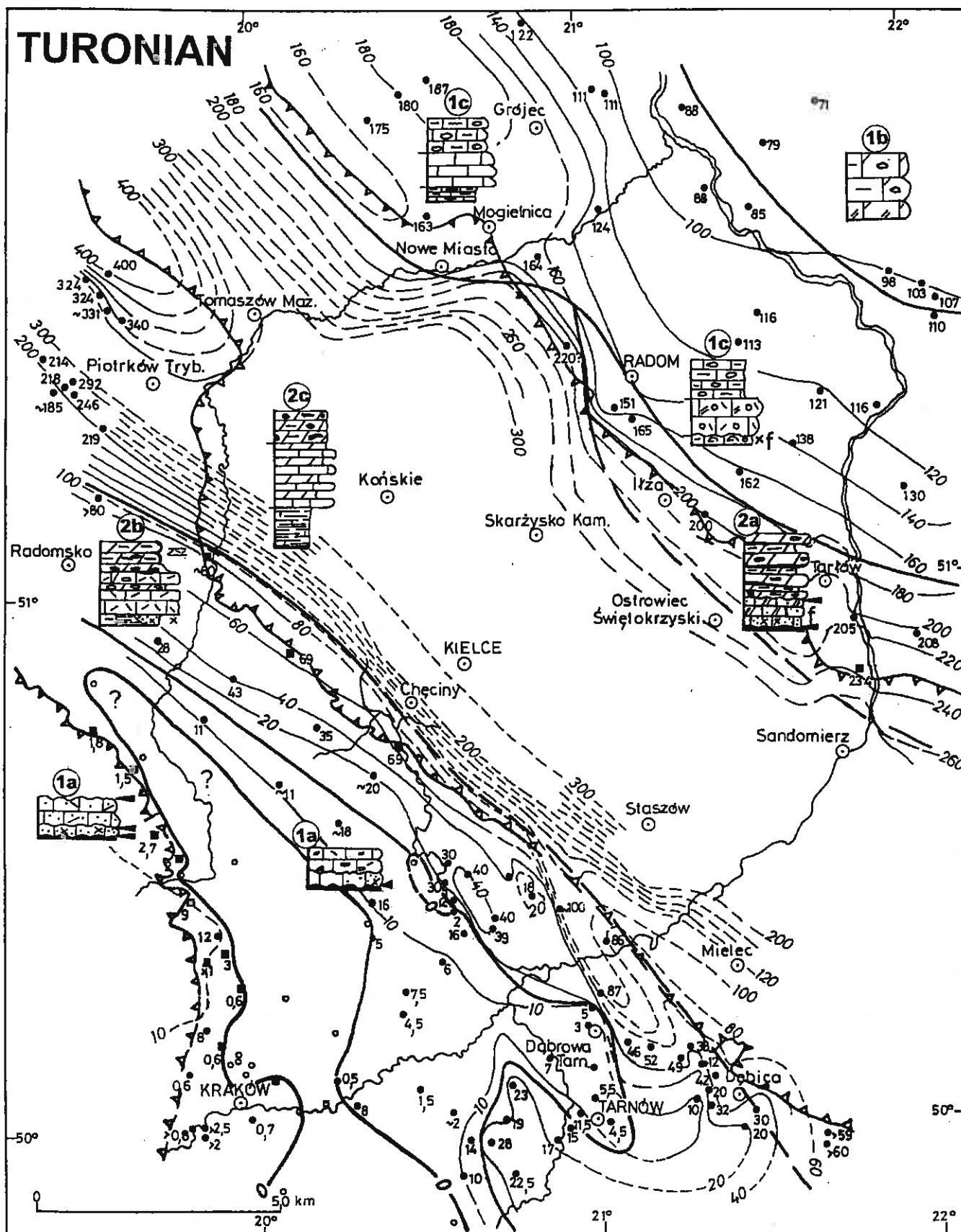
Fig. 6. Thickness and facies patterns of Turonian deposits Explanations see Figs. 1, 2 and 4
