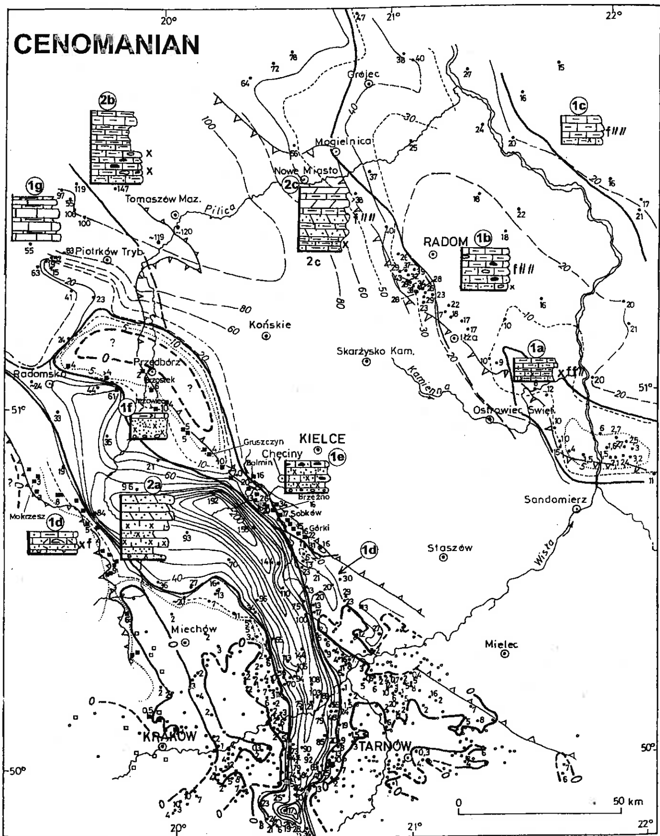
Fig. 5. Thickness and facies patterns of Cenomanian deposits Explanations see Figs. 1, 2 and 4
