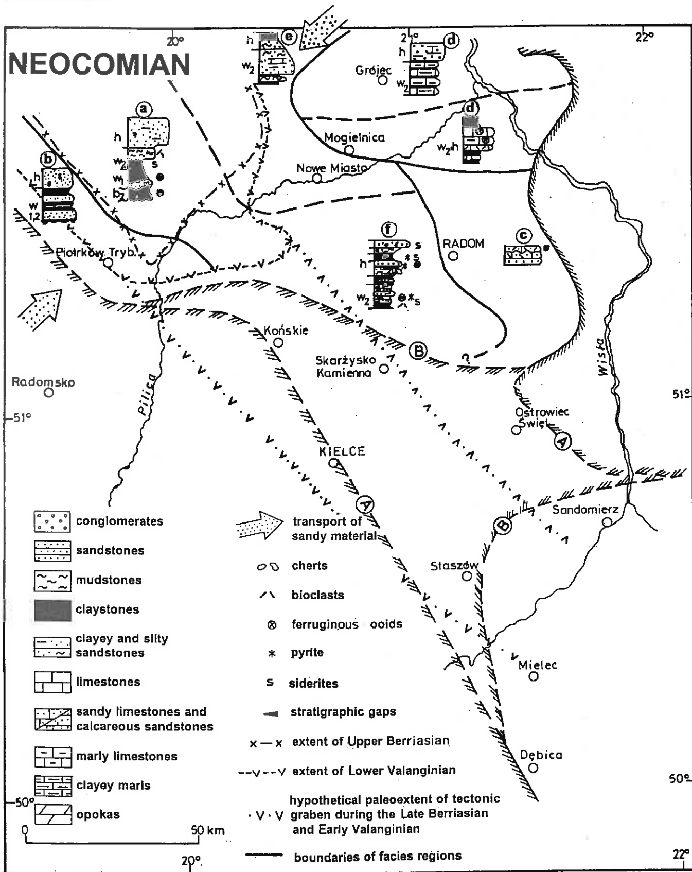
Fig. 2. Facies pattern of Neocomian deposits b2 — Upper Berriasian, w1 — Lower Valanginian, w2 — Upper Valanginian, h — Hauterivian; other explanations see Fig. 1
