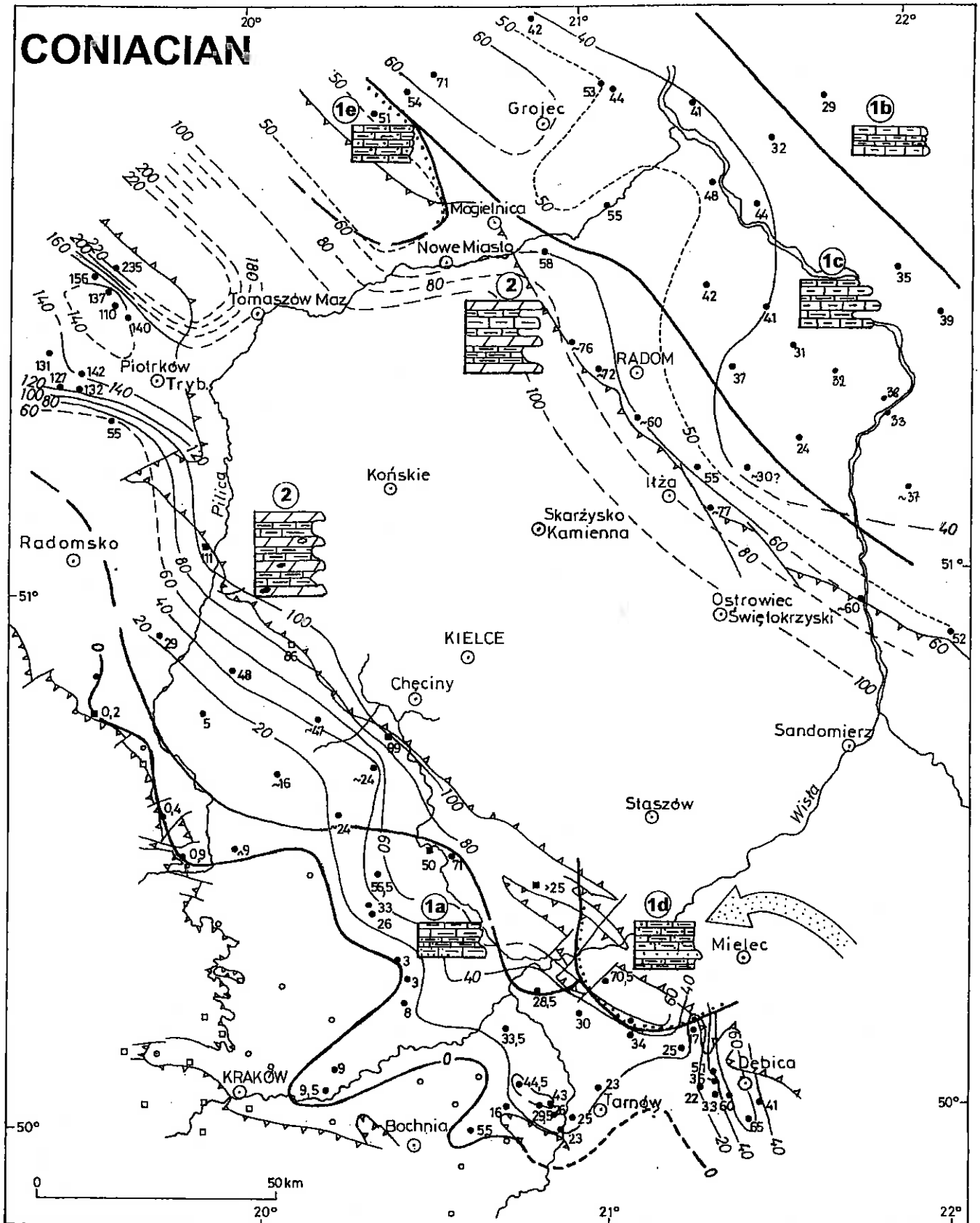
Fig. 7. Thickness and facies patterns of Coniacian deposits
