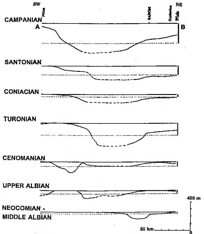
Fig. 12. Palaeotectonic cross-sections of Holy Cross segment of the Mid-Polish Trough
