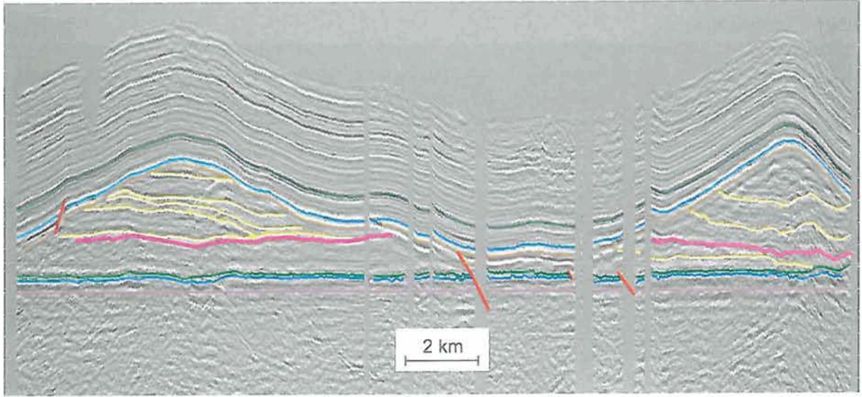
Fig. 5. Interpreted time seismic line 24-5-80K flattened on seismic horizon related to top of the Lower Devonian
