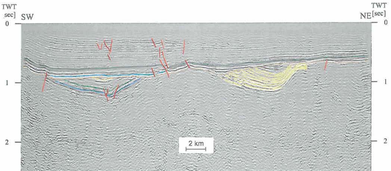
Fig. 6. Interpreted time seismic line 26-5-80K
