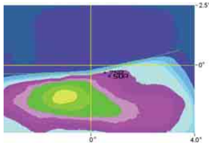
Fig. 5. Illumination distribution for headlamp with random mass production bulb different than for fig. 4. Maximum of illuminance moved far from the 50R and 75R points
