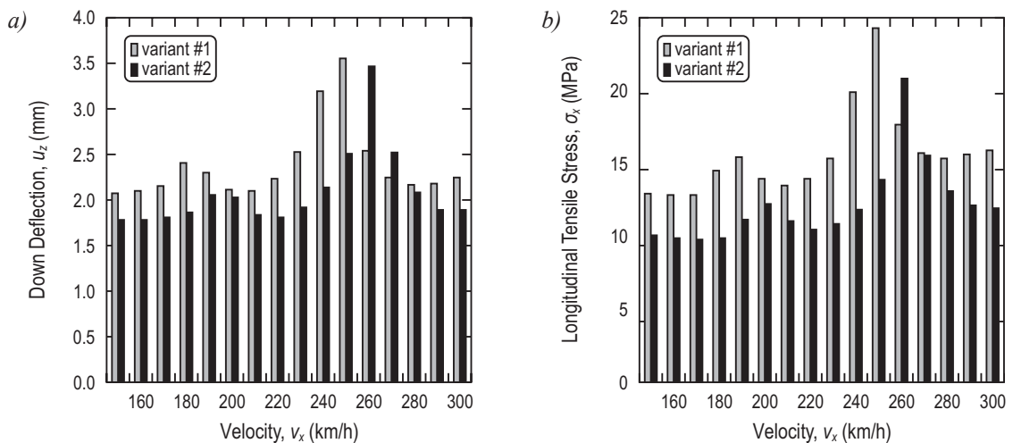
Fig. 15. Comparison of the results for obtained for both variants of the considered viaduct: maximum registered values of deflections (a) and tensile stresses (b)
