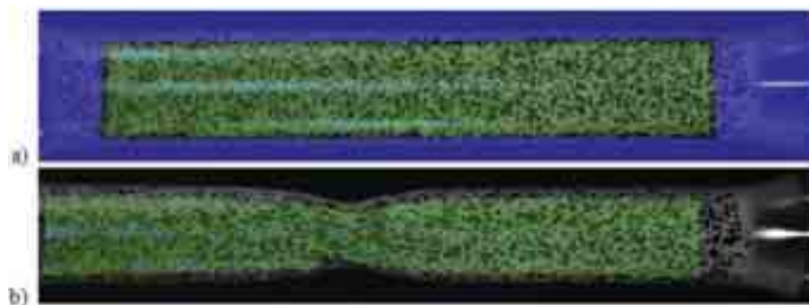
Fig. 3. Picture of the specimen taken by optical system with analysed area marked in green: a) on the beginning of the test and b) one frame before failure
