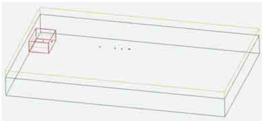
Fig. 2. View of numerical model with visible point of data record and point of excitation
