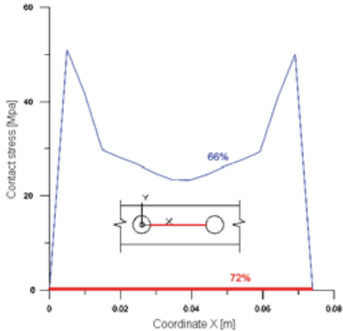
Fig. 8. The distribution of contact stresses, the surface of A and B (0.1 m bolt spacing — 4 scale load)
