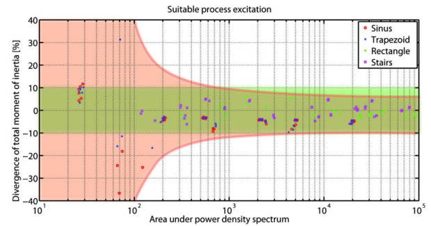
Fig. 8. Divergence of moment of inertia over power density area A_{SUU}
