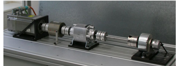
Fig. 3. Test rig with known moment of inertia
