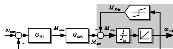
Fig. 2. Scheme of the velocity loop [9] with: \omega_{com} ... command velocity, \omega_{act} ... actual velocity, M_{com} ... command torque, M_{act} ... actual torque, M_{fric} ... friction torque, C_{VC} ... velocity controller, G_{CuL} ... closed current loop
