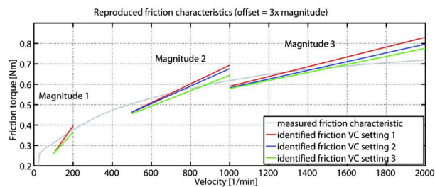
Fig. 6. Identification results for the friction parameters
