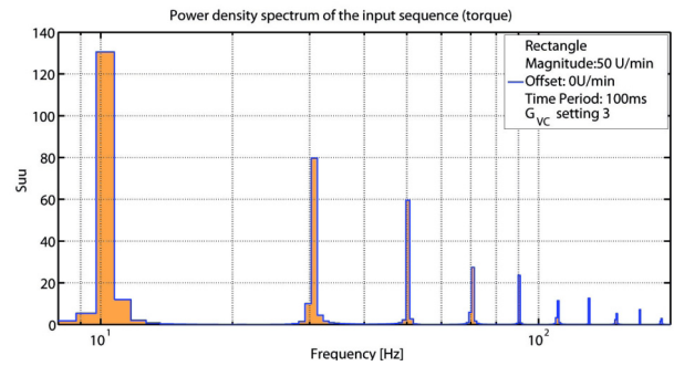
Fig. 7. Power density spectrum of a rectangular input sequence
