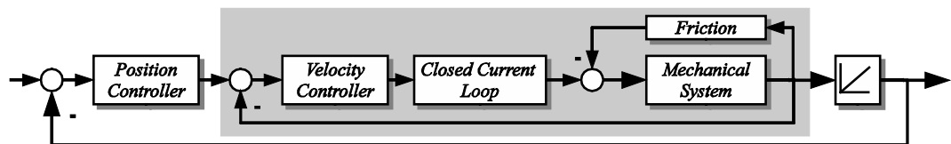
Fig. 1. Cascaded position control with velocity loop (grey)
