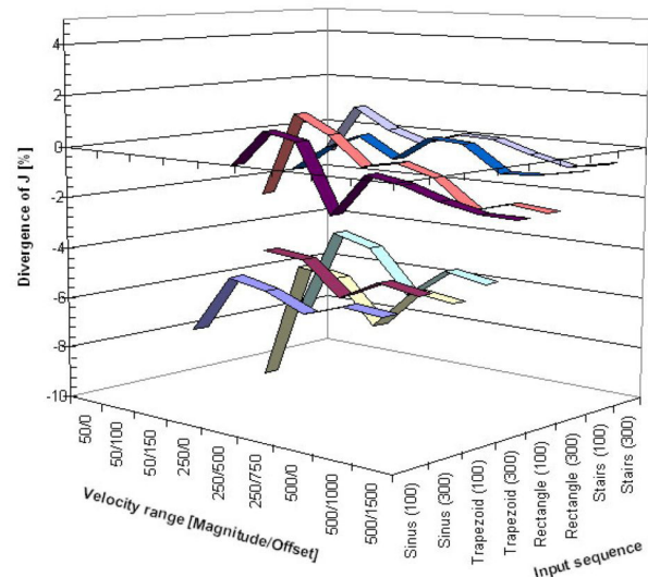
Fig. 5. Identification results for the moment of inertia J_{tot} with velocity controller setting 2
