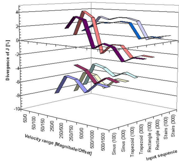
Fig. 4. Identification results for the moment of inertia J_{tot} with velocity controller setting 1
