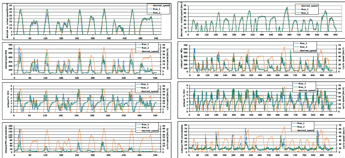
Fig. 5. Comparison of real and desired speed, traces of engine rpm and concentrations of NOx, CO 2 and PM along two consecutive runs of Manhattan Bus Cycle (left) and Orange County Bus Cycle (right). These are presented primarily for demonstration purposes.
