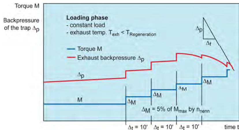
Fig. 8. Regeneration cycle. Plotted are the torque ( M ) steps and the back-pressure ( \Delta p )
