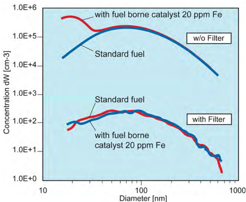
Fig. 6. Bimodal particle distribution, on adding Octimax (a metal-organic fuel-borne catalyst) to standard fuel, with and without filter
