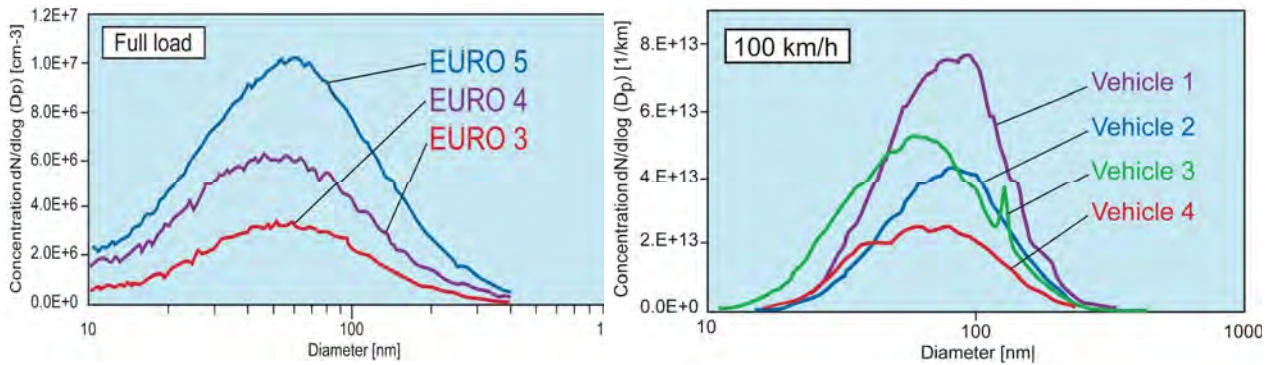
Fig. 2. Particle concentration spectra in the undiluted exhaust-gas
