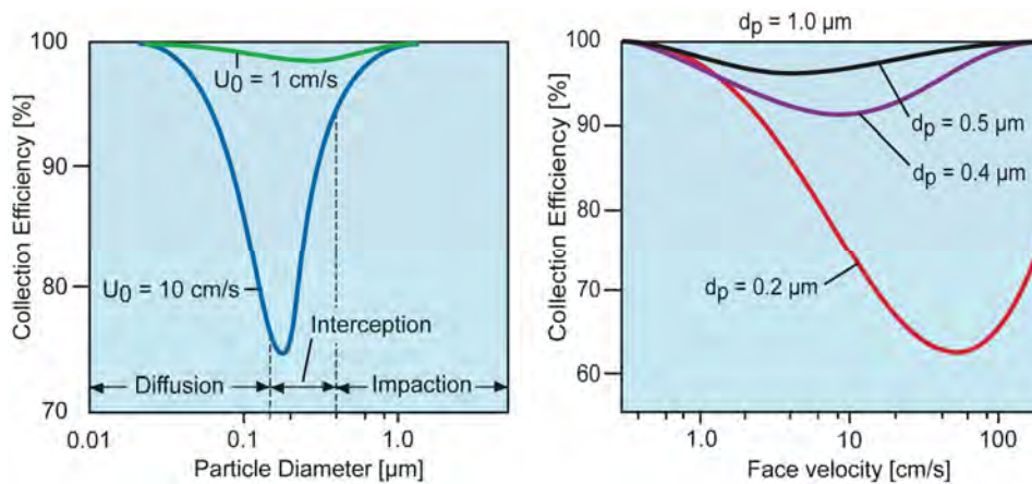
Fig. 3. Filtration efficiency, due to diffusion and impaction, as a function of particle diameter and drag velocity. Hinds [6]
