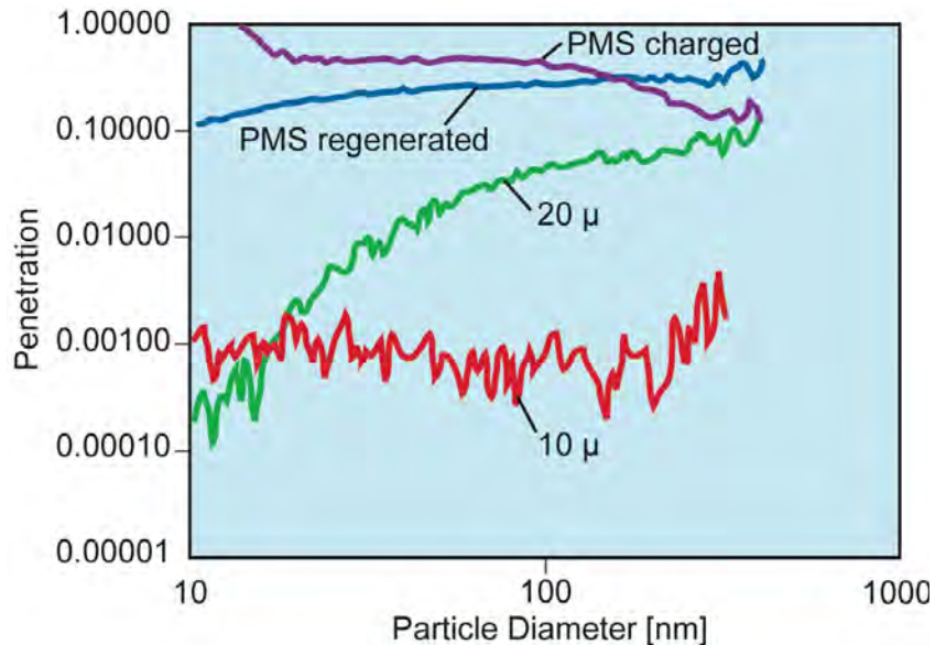
Fig. 5. Penetration characteristic of two wall-flow filters having pore size 10 \mu\text{m} and 20 \mu\text{m} . Also shown are results for an open filter (PMS) in the regenerated and burdened state [16]. Penetration is defined as the ratio of outlet particles to inlet particles. Penetration is thus 1 – filtration efficiency
