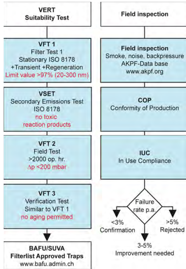
Fig 7. VERT suitability test and field verification
