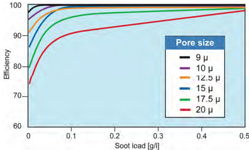
Fig. 4. Filtration efficiency as a function of soot burden and pore size Source: Haus der Technik “Minimierung der Partikelemissionen 2005
