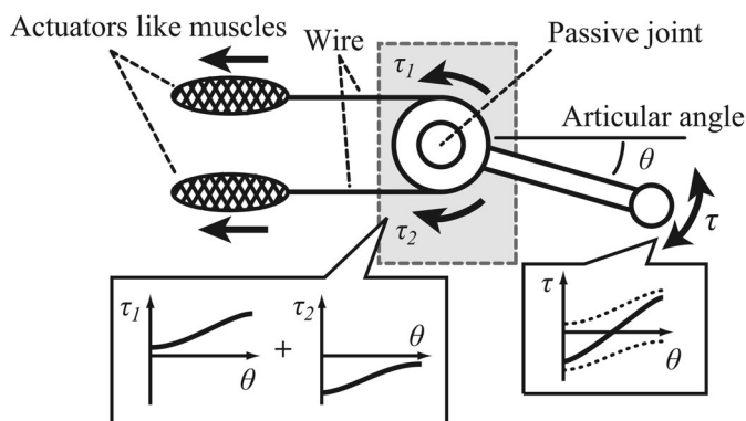
(b) The mechanism using actuators like muscles under the equilibrium point hypothesis.
