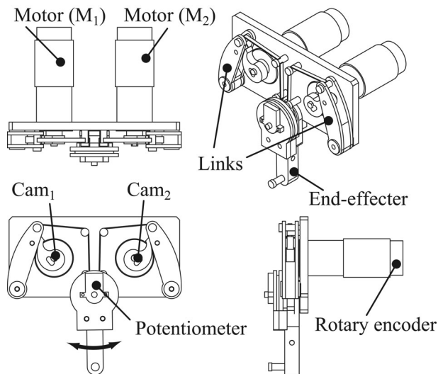
Fig. 10. Antagonized wire-driven mechanism using KTM (1 DOF).
