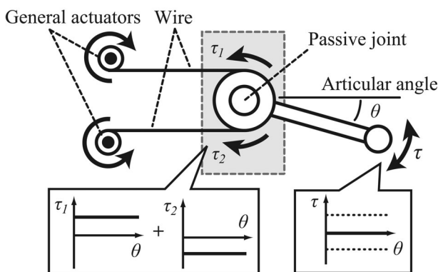
Fig. 4. Wire-driven mechanisms.
