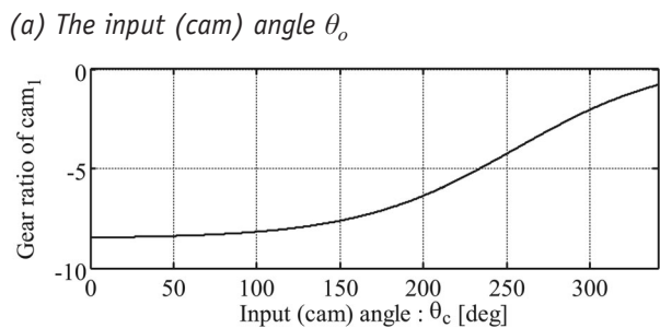
Fig. 8. Gear ratio of designed cam (the case of cam 1 ).
