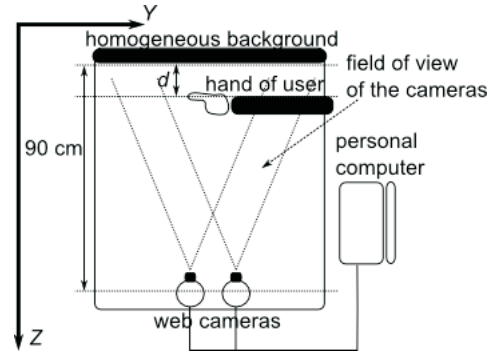
Fig. 3. The experimental setup ( d is the distance of the tip of the index finger from the homogeneous background).
