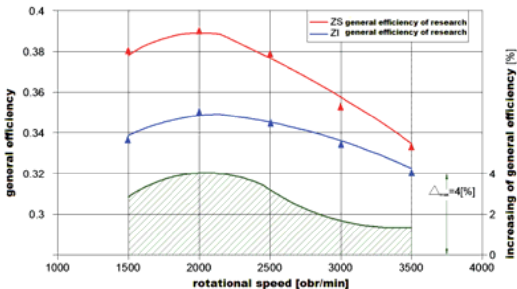
Fig. 9. The course of the increase of the general engine efficiency for the ignition dose determined in relation to the work mode of the spark ignition, set based on test-stand research
