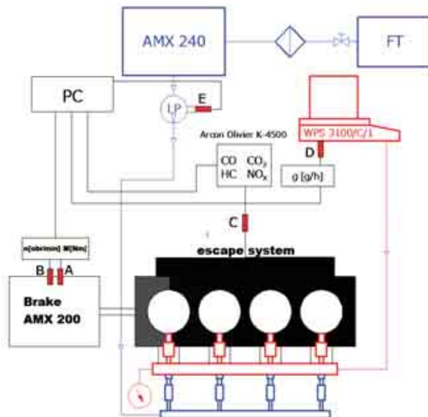
Fig. 1. Diagram of test bed (Symbols: A – measurement of rotational speed, B – measurement of rotational moment, C – measurement of coefficient of air surplus, and toxic components of the exhaust fumes, D – measurement of mass expense of the fuel, for the ignition dose injection, E – measurement of fuel consumption of fundamental dose)
