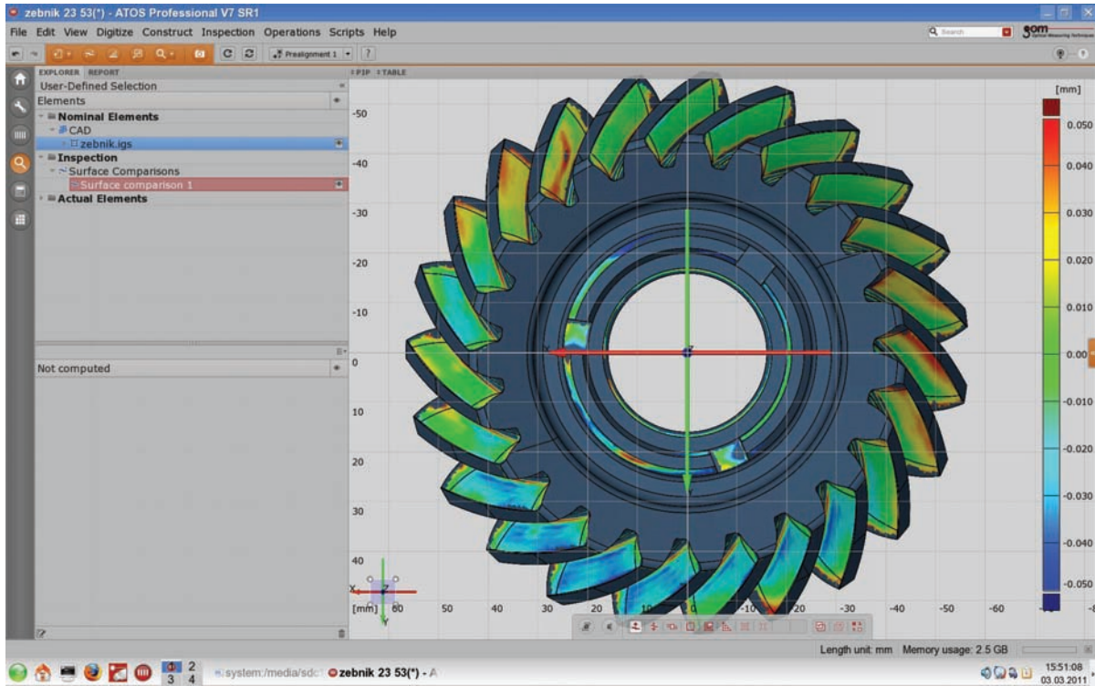
Fig. 6. Analysis of the pinion surface displacement with respect to the CAD model
