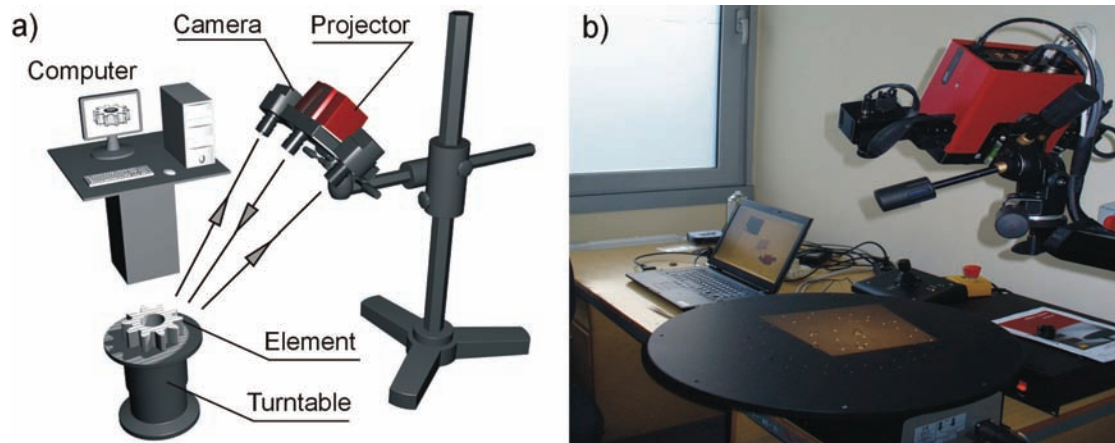
Fig. 1. The measuring system GOM ATOS: a) schema, b) photography
