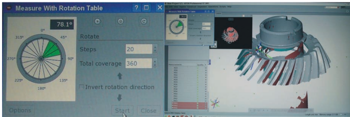
Fig. 4. Measurement pinion using the rotary table – data processing
