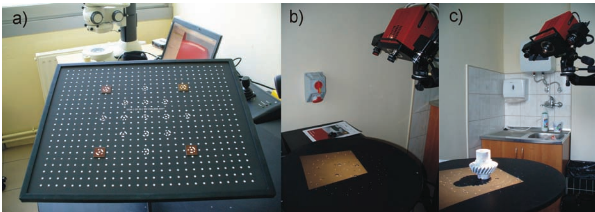
Fig. 3. Measurement with the rotary table: a) calibration, b) turntable calibration, c) measurements of gear
