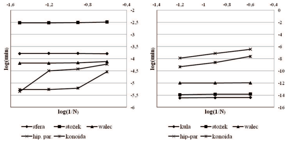
Fig. 32. Inf-sup test – sphere, cone, cylinder, paraboloid, conoid. h_a = 1/100 . S4R Abaqus element. Norm matrix \mathbf{S0} = \mathbf{M} . Full stiffness matrix \mathbf{K} (left) and shear oriented stiffness matrix \mathbf{K}_s (right).
