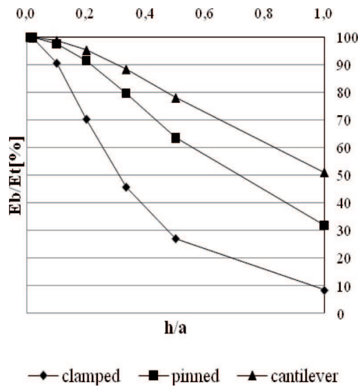
Fig. 9. Bending energy contribution in total energy depending on plate thickness ( h/a=1/100, 1/50, 1/10, 1/5, 1/3, 1/2, \nu=0.3 ).
