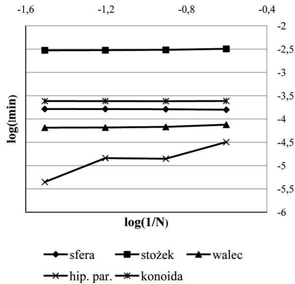
Fig. 30. Inf-sup test – sphere, cone, cylinder, paraboloid, conoid. h_a = 1/100 . S4R5 Abaqus element. Norm matrix S_0 = M . Full stiffness matrix K . Rys. 30. Test inf-sup – sfera, stożek, walec, paraboloida, konoida. h_a = 1/100 . Element Abaqus S4R5. Macierz normowa S_0 = M . Pełna macierz sztywności K
