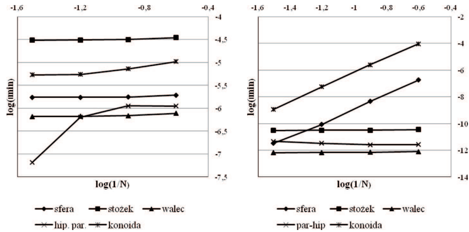
Fig. 33. Inf-sup test – sphere, cone, cylinder, paraboloid, conoid. h_a = 1/1000 . S4 Abaqus element. Norm matrix \mathbf{S0} = \mathbf{M} . Full stiffness matrix \mathbf{K} (left) and shear/membrane oriented stiffness matrix \mathbf{K}_{sm} (right).
