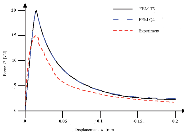
Fig. 17. Nooru-Mohamed [33] test: calculated force-displacement curves for 2 different FE element types at P_s = 5 kN compared with experiment (using model by Cox [26]).
