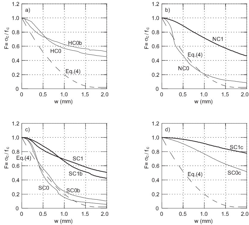
Fig. 9. The F(w) curves resulting from triaxial tests: a) specimens made of HPFRCC; b) specimens made of NC; c) specimens made of SC-mix1 and SC-mix1; d) specimens made of SC-mix3.
