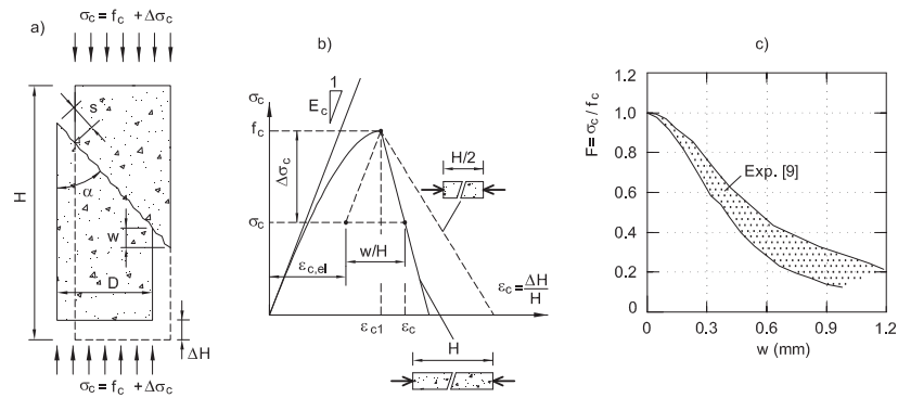
Fig. 4. The post-peak response of quasi-brittle materials in compression: a) sliding of the damaged specimen; b) possible stress-strain curves; c) the non-dimensional function F(w) measured by Jansen and Shah [9].
