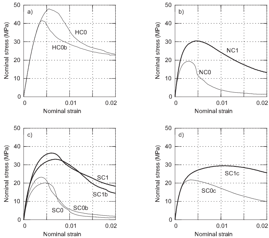
Fig. 8. The stress-strain curves resulting from triaxial tests: a) specimens made of HPCFRCC; b) specimens made of NC; c) specimens made of SC-mix1 and SC-mix1; d) specimens made of SC-mix3.
