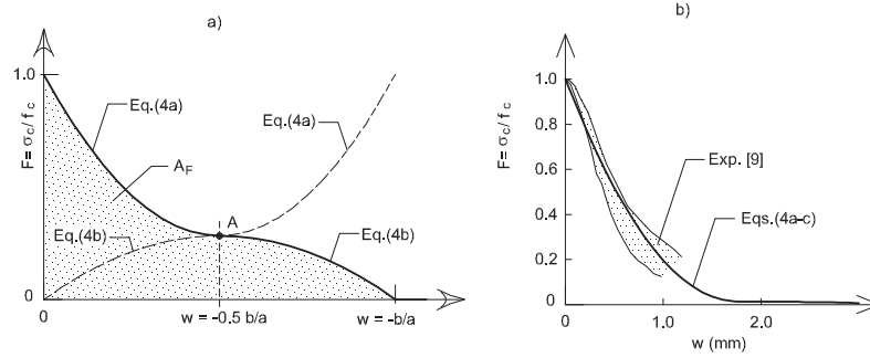
Fig. 5. Modelling the post-peak response under compression: a) The stress-inelastic displacement relationship proposed by Fantilli et al. [10]; b) the F(w) relationship in the case of normal vibrated concrete.
