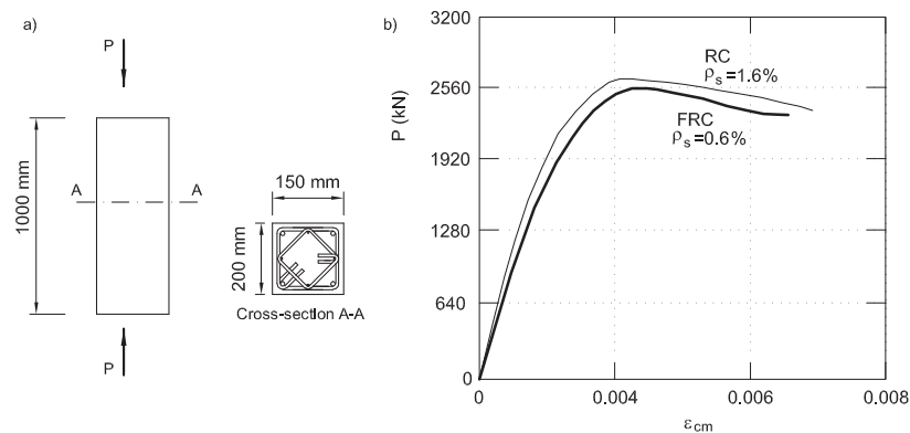
Fig. 3. The tests by Ganesan and Ramana Murthy [5]; a) geometry of the columns; b) load v.s. average strain curves.
