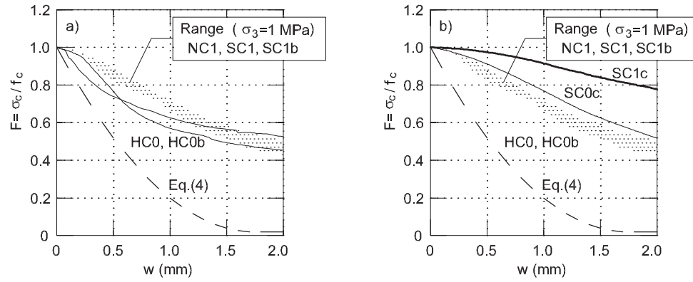
Fig. 10. The active confinement of high performance concretes: a) the F(w) curves of HPRC; b) the F(w) curves of SC-mix3.
