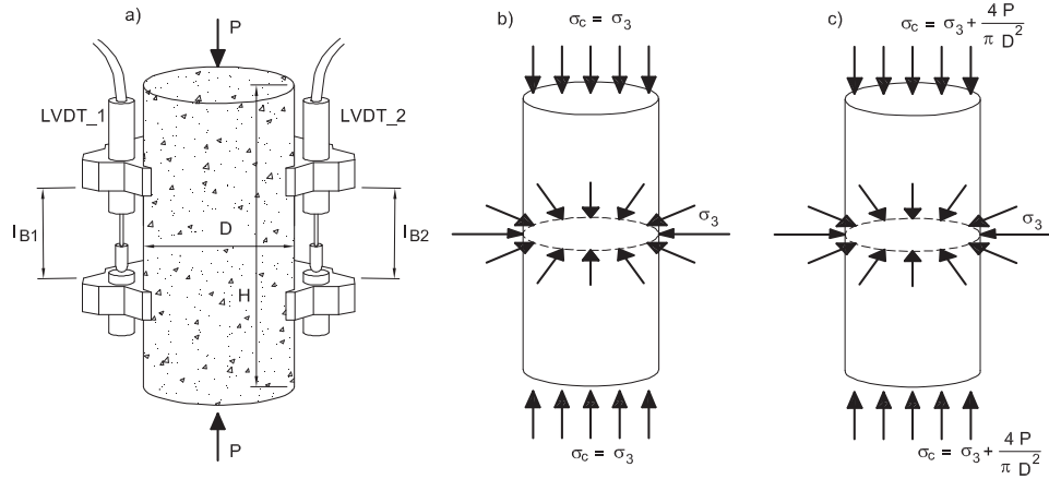
Fig. 6. Triaxial tests performed at Politecnico di Torino (Italy): a) position of the LVDTs; b) first stage of loading; c) second stage of loading.
