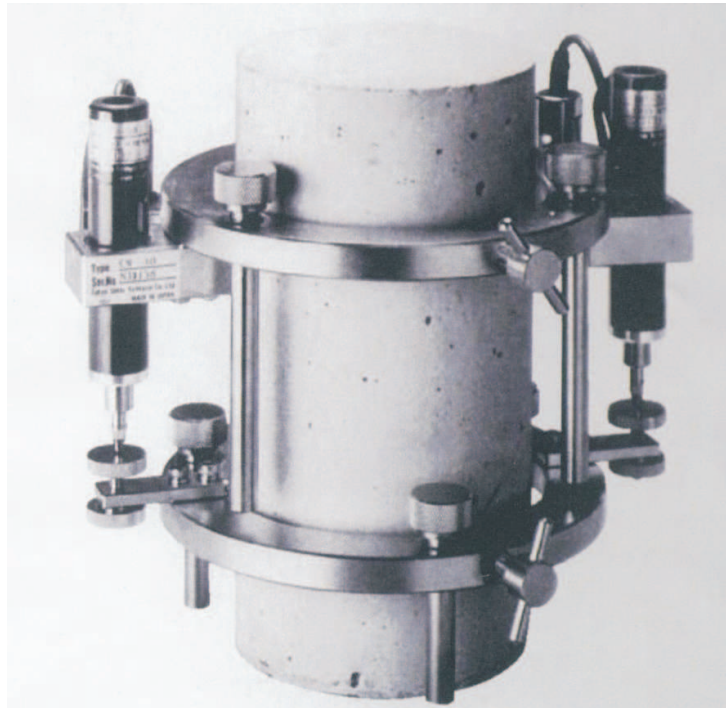
Fig. 7. Position of the LVDTs in the uniaxial tests performed at Tohoku University (Japan).
