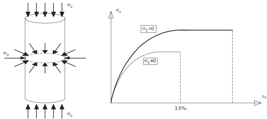
Fig. 2. The stress-strain relationship of compressed concrete with and without confinement [4].
