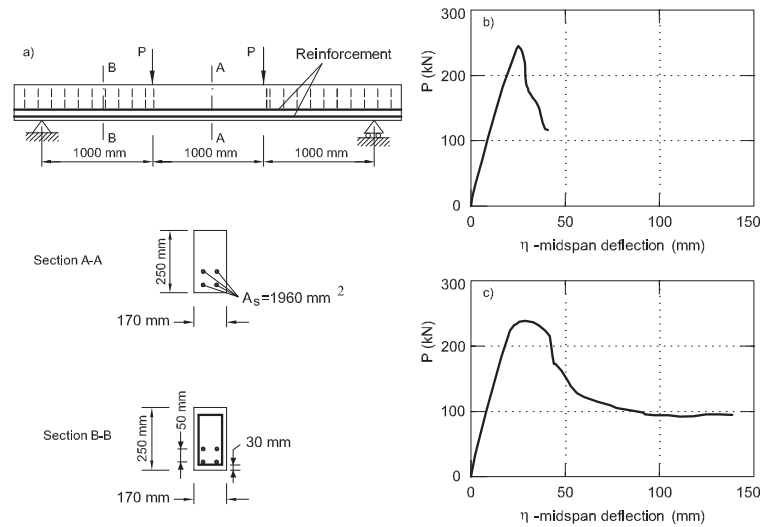
Fig. 1. The tests performed by Mansur et al. [1]: a) geometrical properties of beams tested in four point bending; b) mechanical response of plain RC beam; c) mechanical response of fiber-reinforced RC beam.
