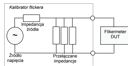
Rys. 3. Schemat kalibratora flikera Fig. 3. Flicker Calibrator functional diagram
