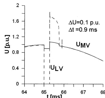
Fig. 7. Fault clearing time with the CHCL (simulation)
