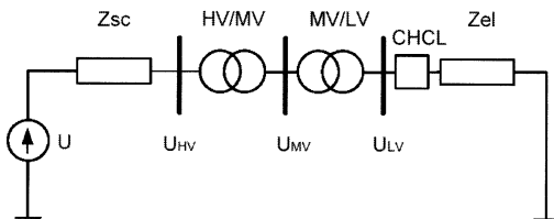
Fig. 4. The modelled power-system grid segment: U - the voltage source, Z_{sc} - the system impedance, HV/MV, MV/LV - the transformer, Z_{el} - the load impedance
