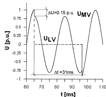
Fig. 6. Fault clearing time with a contact switch (simulation)
