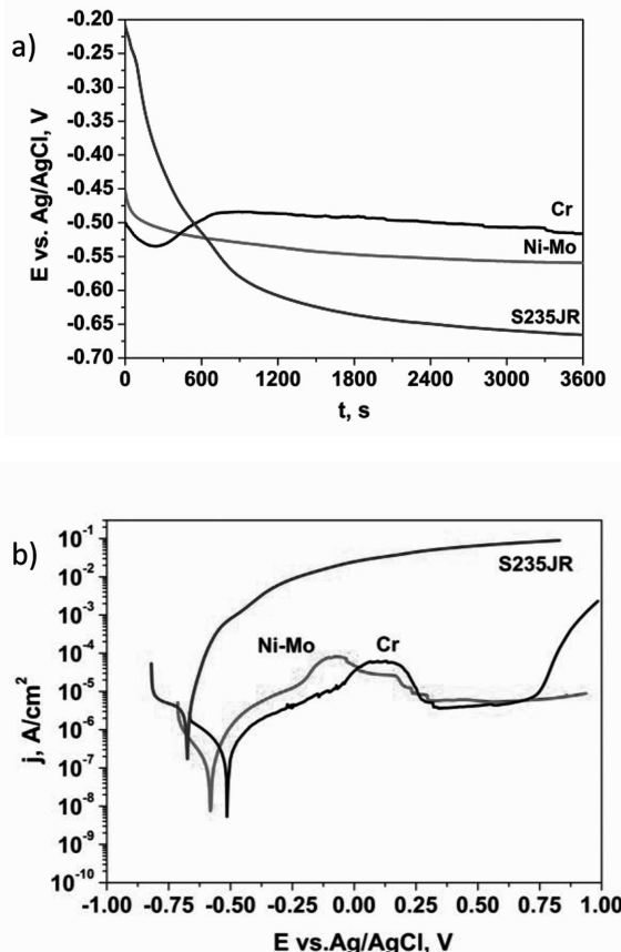
Fig. 11. a) Corrosion potential vs. Ag/AgCl reference electrode as a function of time, b) polarization curves of Ni-Mo, Cr and steel substrate (S235JR) in 0.5M Na 2 SO 4
