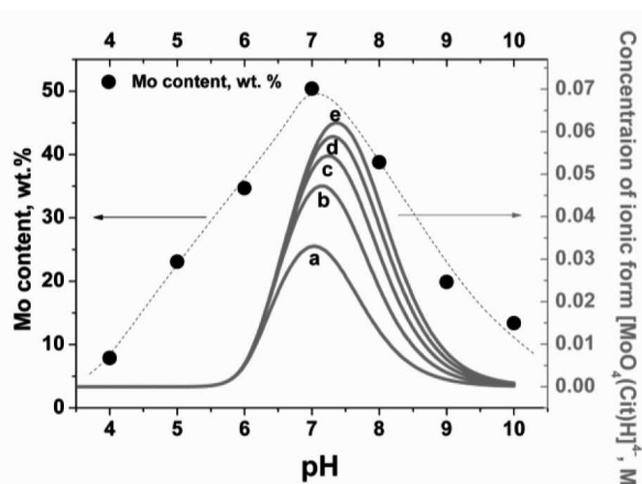
Fig. 1. Molybdenum content in Ni-Mo alloys electrodeposited at j = 2.5 A/dm 2 and concentration of the electroactive molybdenum species [\text{MoO}_4(\text{Cit})\text{H}]^{4-} in solution, calculated for the following molar ratio [\text{Mo(VI)}]:[\text{Cit}] : a) 1:1, b) 1:2, c) 1:3, d) 1:4, e) 1:5 as a function of pH (Cit=C 6 H 5 O 7 3- )
