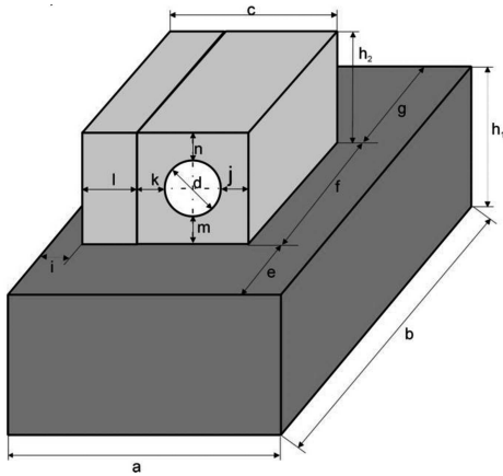
Fig. 3. Symbols of dimensions of induction heater
