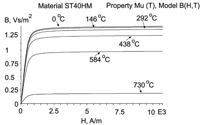
Fig. 4. Magnetization characteristic of the used material (steel 40HM) for different temperatures
