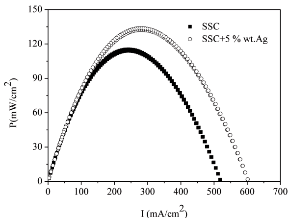
Fig. 11. The family of P-I curves recorded for IT-SOFC with \text{Ce}_{0.78}\text{Sr}_{0.02}\text{Gd}_{0.2}\text{O}_2 as a solid electrolyte with monophasic cathode \text{Sm}_{0.5}\text{Sr}_{0.5}\text{CoO}_3 (SSC) or \text{Sm}_{0.5}\text{Sr}_{0.5}\text{CoO}_3 +5% wt.Ag at temperature 700^\circ\text{C}
