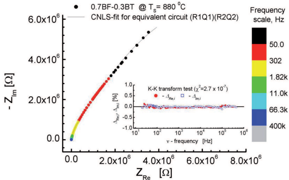
Fig. 11. Impedance diagram for 0.7BF–0.3BT ceramic sintered at T=880^{\circ}\text{C} (method III) and Kramers-Kronig test of impedance data
