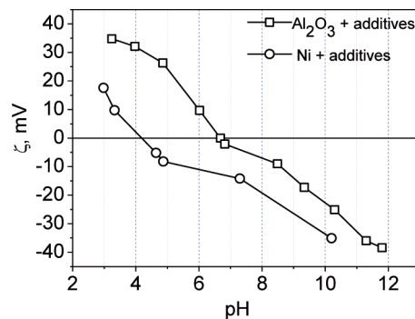
Fig. 3. Zeta potential as a function of pH of Al_2O_3 and Ni powders with additives
