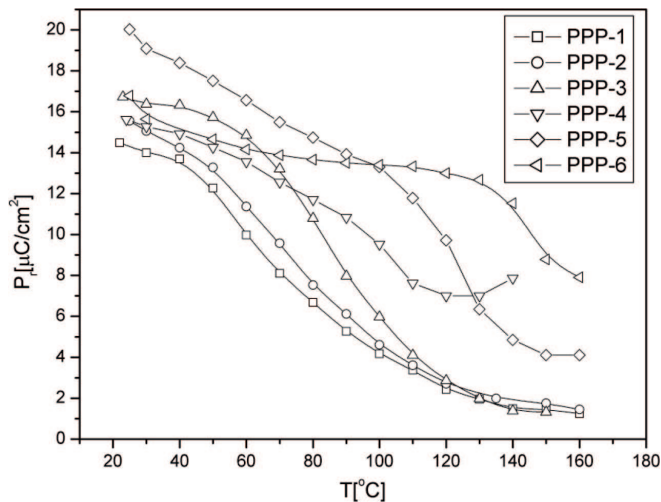
Fig. 7. The dependency of remnant polarization P_r on temperature for all investigated samples
