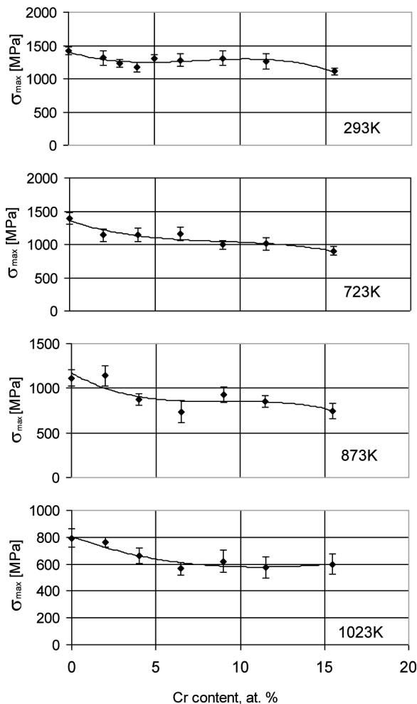
Fig. 2. The values of maximum true stress \sigma_{max} for the Ni 75 Al (25-x) Cr x alloys
