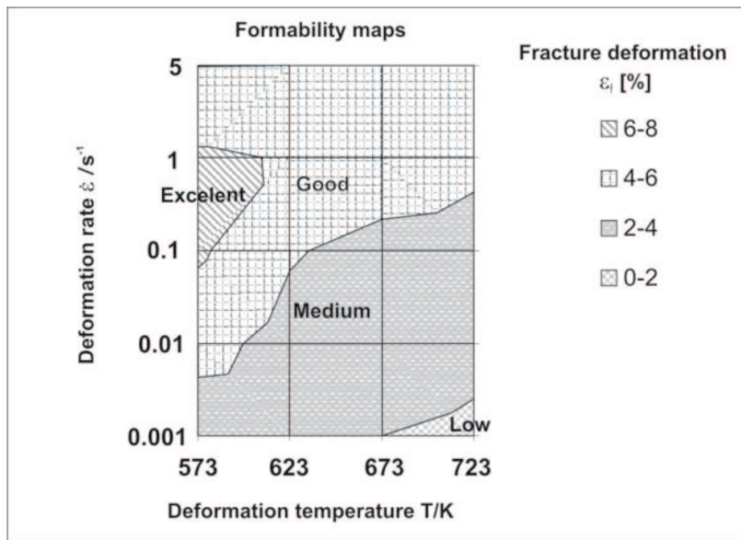
Fig. 6. Formability maps for investigated alloy
