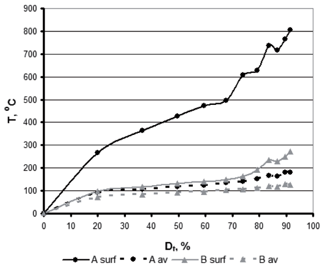
Fig. 6. The change of temperature on the surface and the axis after exit from the bearing zone of die for wires drawn according to variant A and B in total draft function
