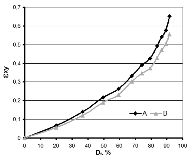
Fig. 8. The change of redundant strain \varepsilon_{xy} of wire surface in total draft function for variant A and B
