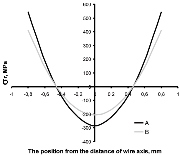
Fig. 4. The distribution of the first type longitudinal residual stresses \sigma_r for \phi 1.6 mm wires drawn according to variant A (classical dies) and B (hydrodynamic dies)
