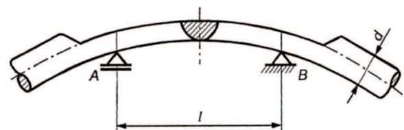
Fig. 1. The deformation of wires after longitudinal grinding to the half diameter [8]
