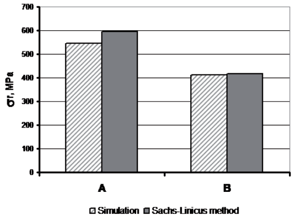
Fig. 5. The values of the first type longitudinal residual stresses \sigma_r on the surface for \phi 1.6 mm wires drawn according to variants A (classical dies) and B (hydrodynamic dies)
