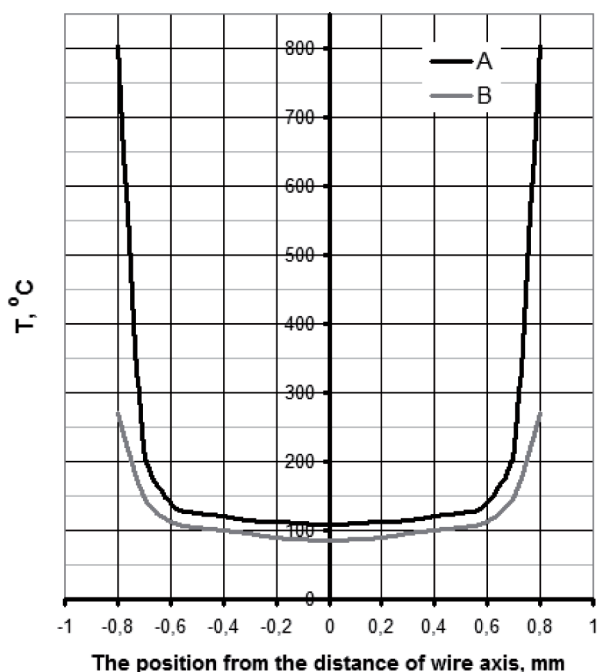
Fig. 7. The distribution of temperature on the cross-section of \phi 1.6 mm wires drawn according to Variants A and B after exit from the bearing zone of die
