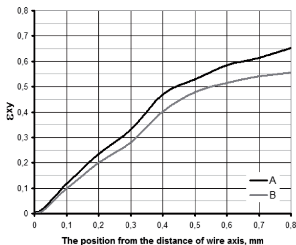
Fig. 9. The distributions of the redundant strain \varepsilon_{xy} on the cross-section of \phi 1.6 mm wires drawn according to Variants A and B
