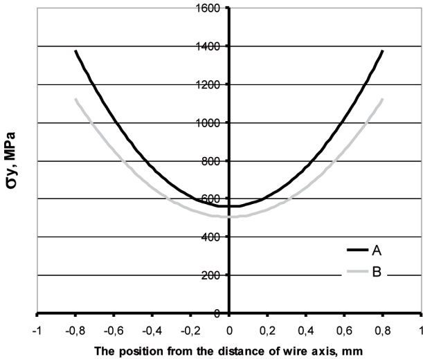
Fig. 3. The distribution of the longitudinal stresses \sigma_y for \phi 1.6 mm wires drawn according to variant A (classical dies) and B (hydrodynamic dies)
