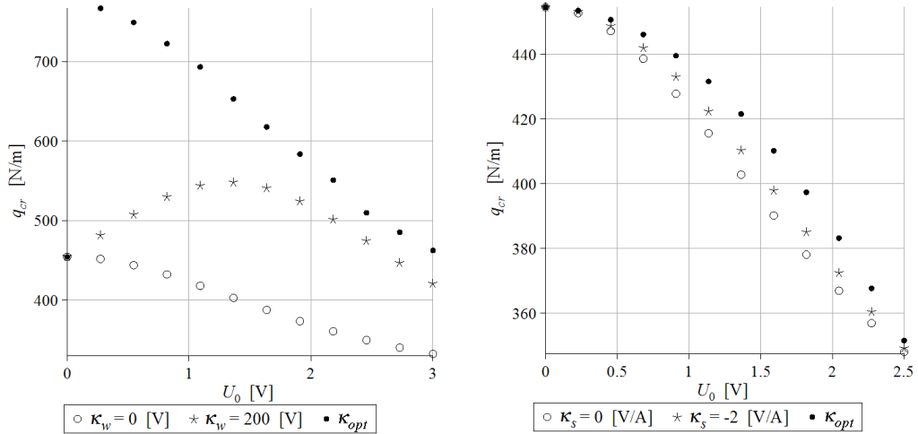
Figure 10. Critical tensional load for the control depending on the displacement (on the left) and on the current (simple one, right), x_e = 0.33L , air.
