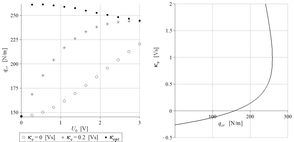
Figure 3. Critical compressive load for the control depending on velocity and without active control (on the left) and the relation between this load and the control for U_0 = 1 V (right), x_e = 0.33L , air.
