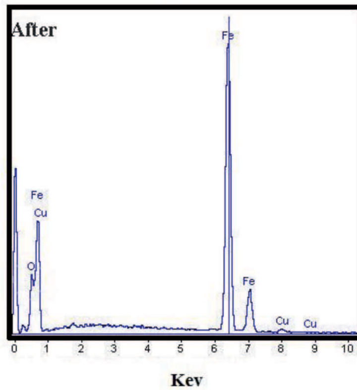
Fig. 6. Typical EDS analysis of worn surfaces (a) PM1 (b) PM4
