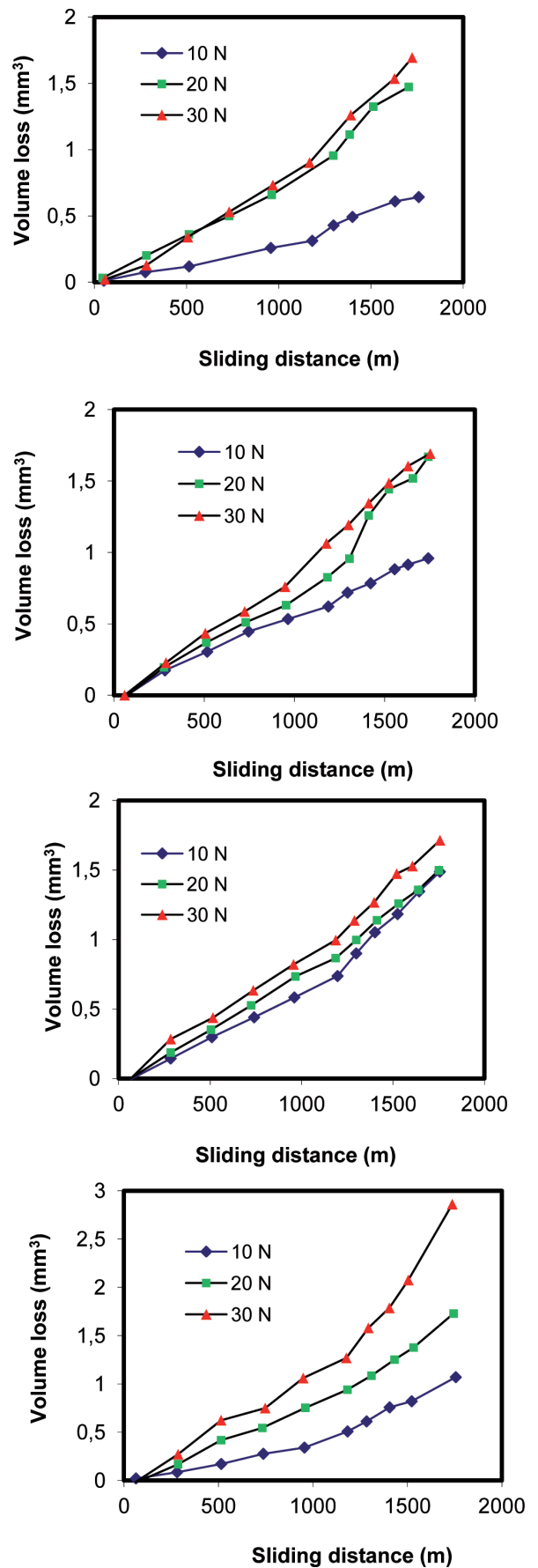
Fig. 4. The variations of volume loss with the sliding distance: (a) PM1; (b) PM2; (c) PM3; (d) PM4
