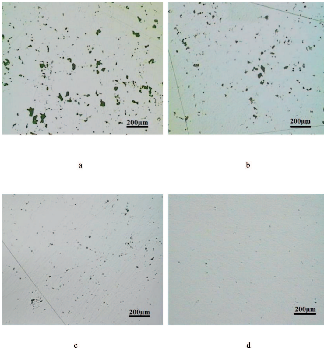
Fig. 1. Microstructure of the studied materials: (a) PM1; (b) PM2; (c) PM3; (d) PM4
