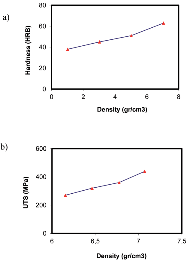
Fig. 2. The effect of density on: (a) HRB, (b) UTS
