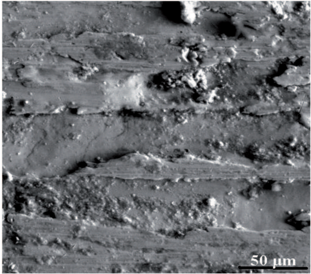
Fig. 8. Typical micrographs of a worn specimen (a) PM1, (b) PM2
