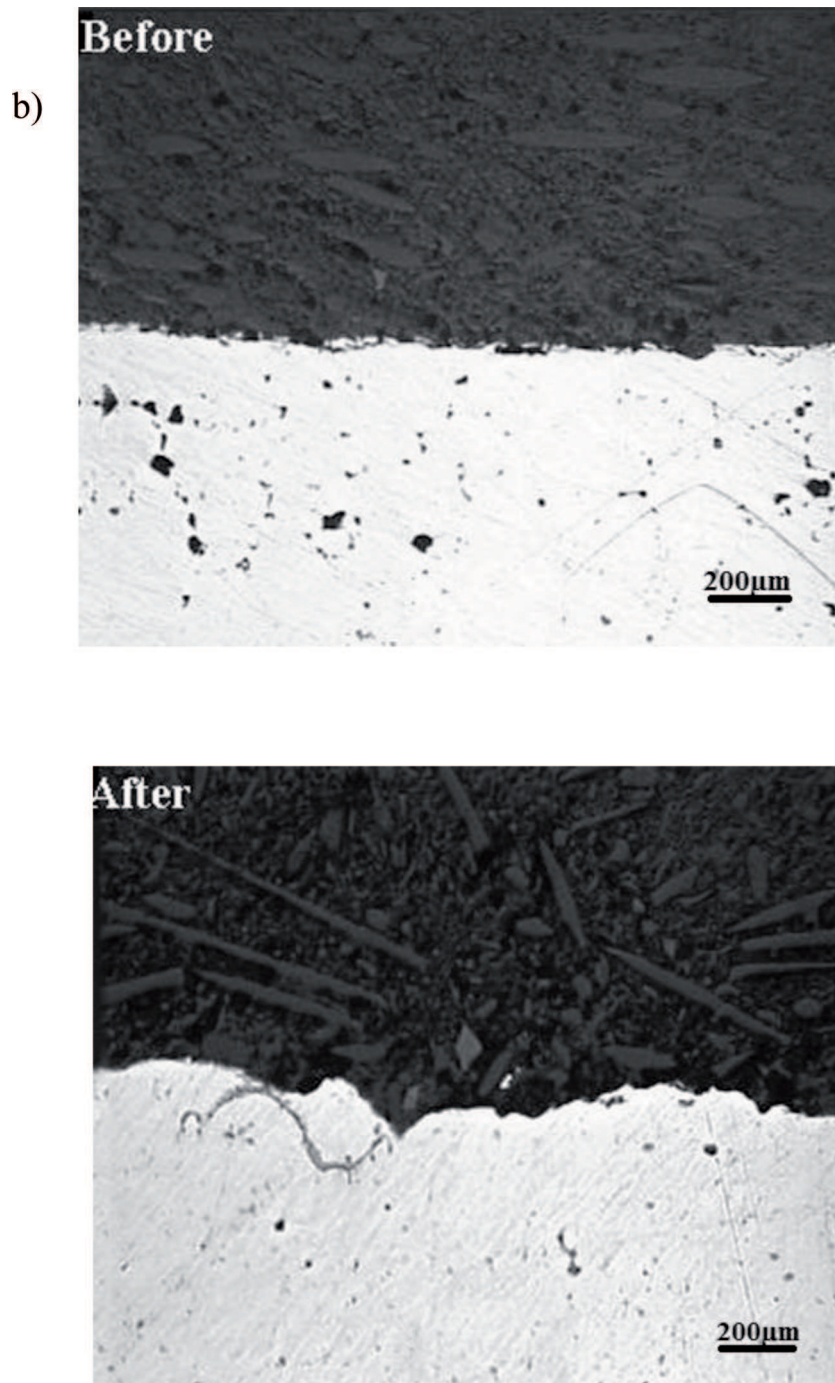
Fig. 5. Typical cross-section micrographs of a worn specimen before and after wear: (a) PM1, (b) PM3
