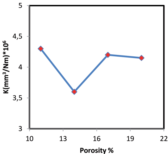
Fig. 9. The variations of volume loss with porosity (Applied load: 20 N)
