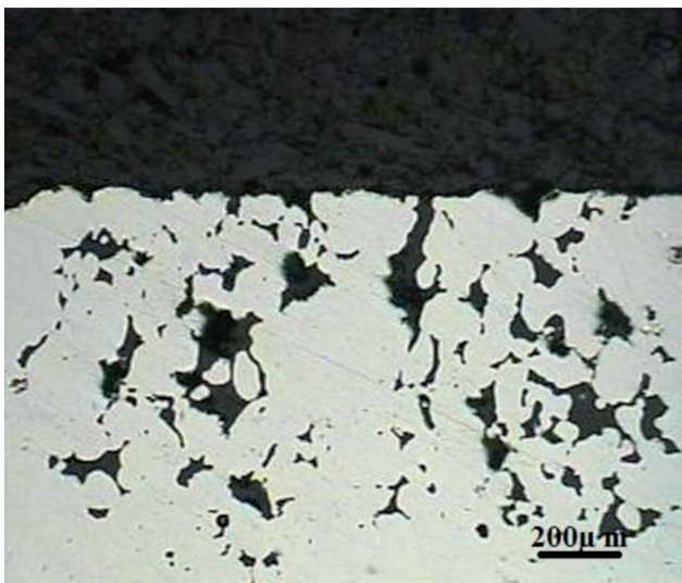
Fig. 3. Typical cross-section micrograph showing pores at the surface of the of sintered samples
