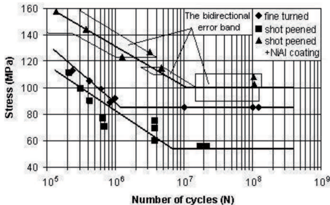
Fig. 2. S-N curves of the tested specimens (Mg-Al-Zn-Mn alloy): with fine turned surface, with the shot peened surface, with the shot peened surface and NiAl coating
