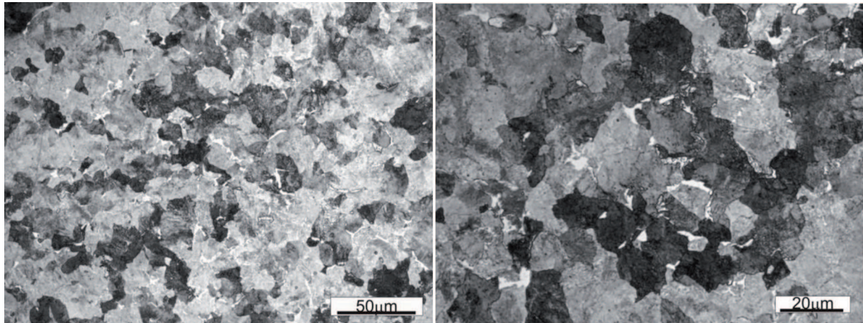
Fig. 1. Microstructure of the tested tyre steel
