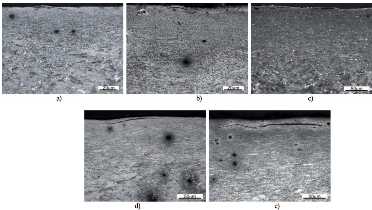
Fig. 9. Morphology of the near-to-surface layer of specimens made of the tested tyre steel (after a tribological test). The cross-sections were made perpendicular to the rolling direction: a) slippage 0.23%, rotational speed 300 rpm; b) slippage 0.5%, rotational speed 100 rpm; c) slippage 1.5%, rotational speed 200 rpm; d) slippage 5%, rotational speed 100 rpm; e) slippage 5%, rotational speed 300 rpm
