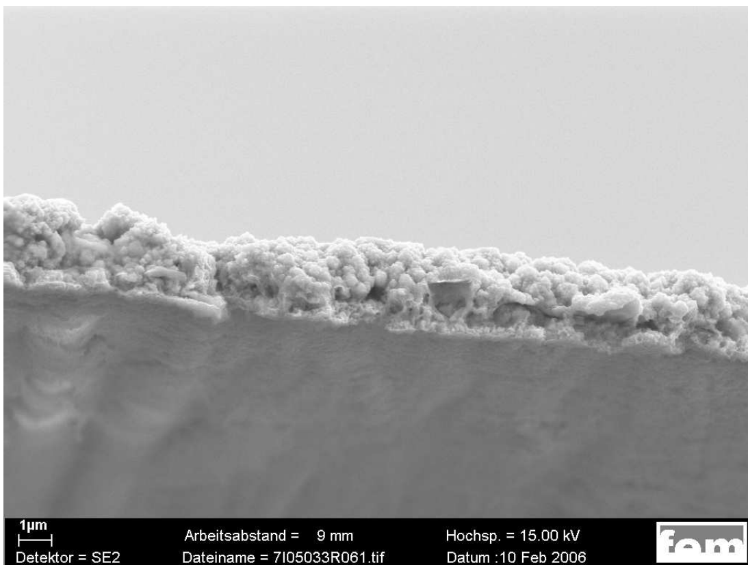
Fig. 4c. SEM image of the cross-section of sample B
