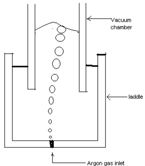
Fig. 2. Schematic diagram of REDA process
