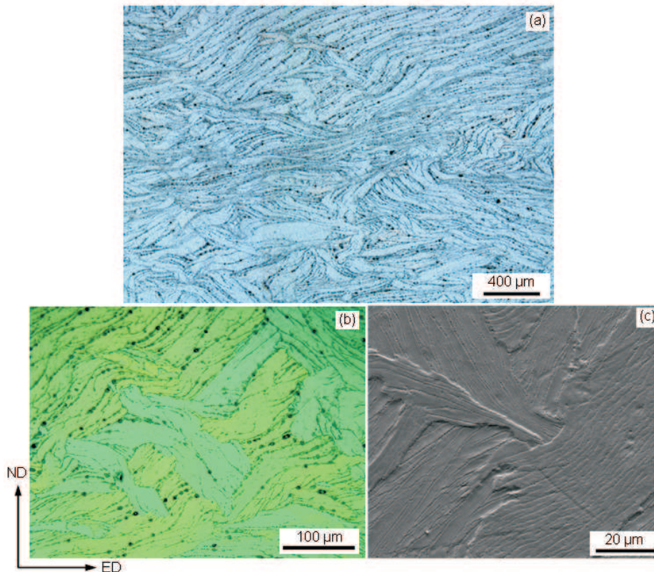
Fig. 1. Typical microstructure of \beta -quiet material after plane strain compression. (a) Optical micrographs showing laths microkinking. Analyses at larger magnification show localization of precipitates in lath boundaries; (b) microstructure after electrolytic polishing observed under polarized light in optical microscopy and (c) SEM observations in secondary electrons. The contrast obtained in polarized light shows different orientations of the \alpha -grains. Sections perpendicular to TD. Sample deformed up to 0.2 (logarithmic strains) at 750°C and strain rate 1s^{-1}
