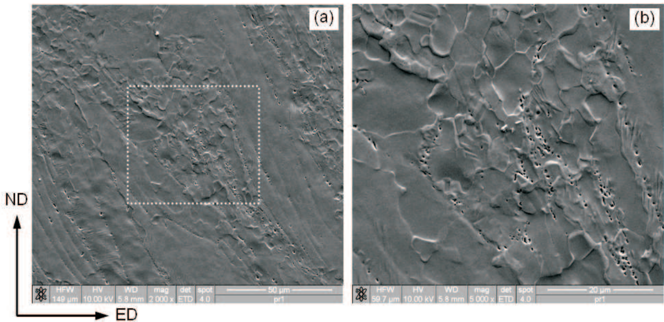
Fig. 3. Beginning stage of recrystallization in near surface region of the sample deformed at 750°C and strain rate of 0.01\text{s}^{-1} . Microstructure observed by using SEMFEG in secondary electrons on sample deformed up to logarithmic strains of 0.5 in channel-die
