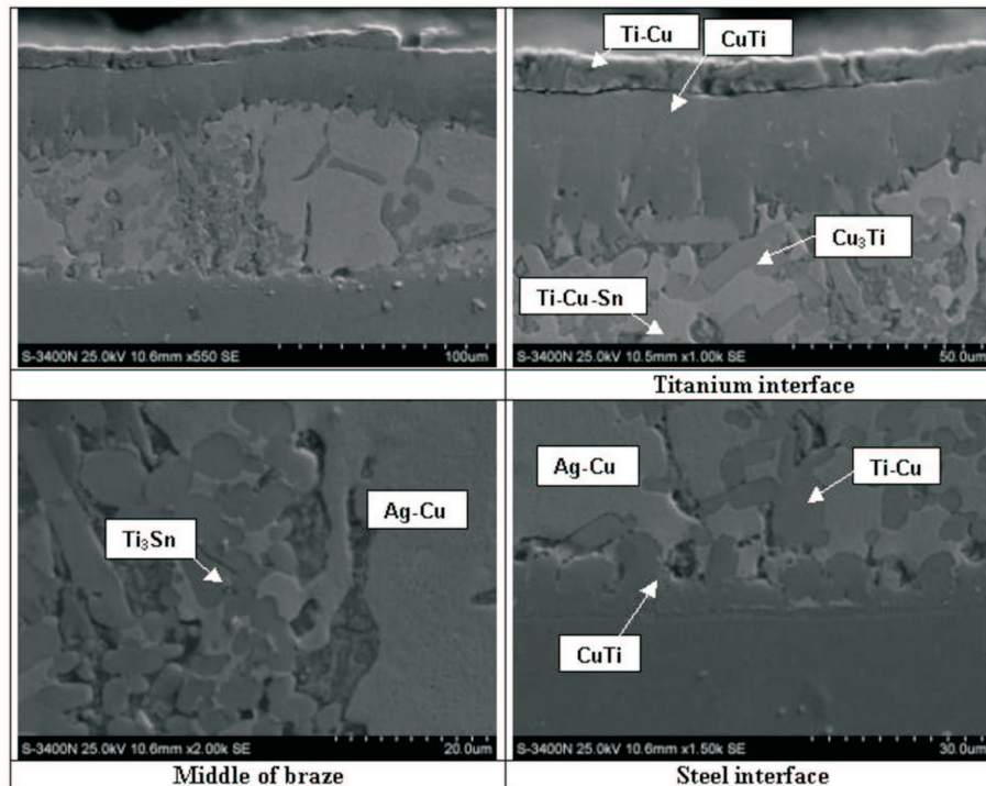
Fig. 6. Microstructure of stainless steel – titanium joint brazed with B-Ag68CuSn-730/755 (Ag68Cu28Sn4) silver brazing alloy at temperature 900°C, SEM
