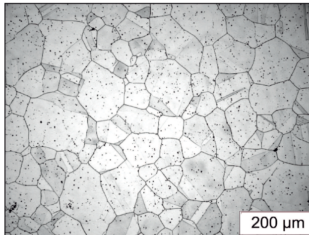
Fig. 1. Microstructures of the investigated steel after solution heat treatment at 1150°C 1h
