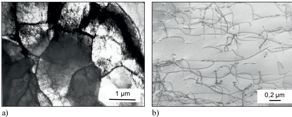
Fig. 9. Substructure after hot deformation at 1000^{\circ}\text{C}/0.01\text{ s}^{-1} to strain \varepsilon = : a) well-defined subgrain, b) example of an image that was used for determination of the dislocation density
