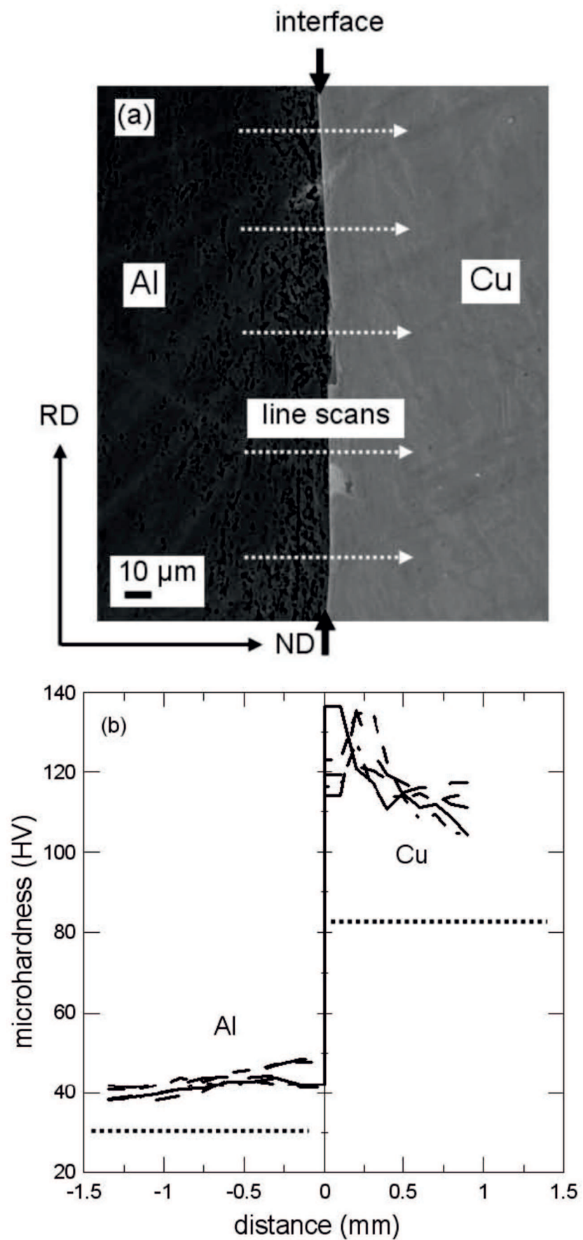
Fig. 3. Vickers microhardness line scans across the Cu/Al interface in areas without melted volumes. Dotted lines mark the average microhardness of fully recrystallized (initial) sheets
