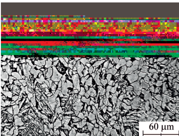
Fig. 4. The microstructure of the specimen after rolling simulation according to scheme 2 from Table 2
