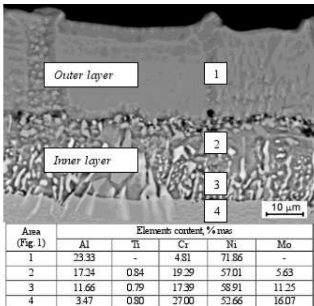
Fig. 1. Microstructure of aluminide coating on IN713LC obtained in a low activity CVD process at the temperature 1050°C for 8h and corresponding chemical compositions in the areas marked in the figure
