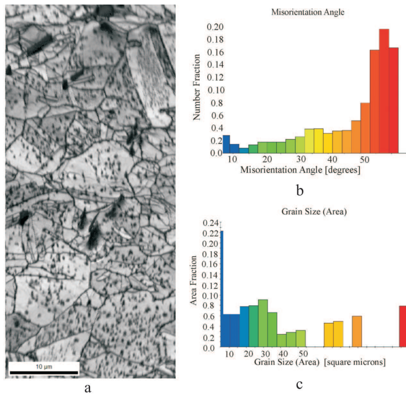
Fig. 5. Microstructure of CuCr alloy strip after 34 passes of deformation (a), with grain boundaries disorientation (b) and grain size distribution (c), SEM with EBSD
