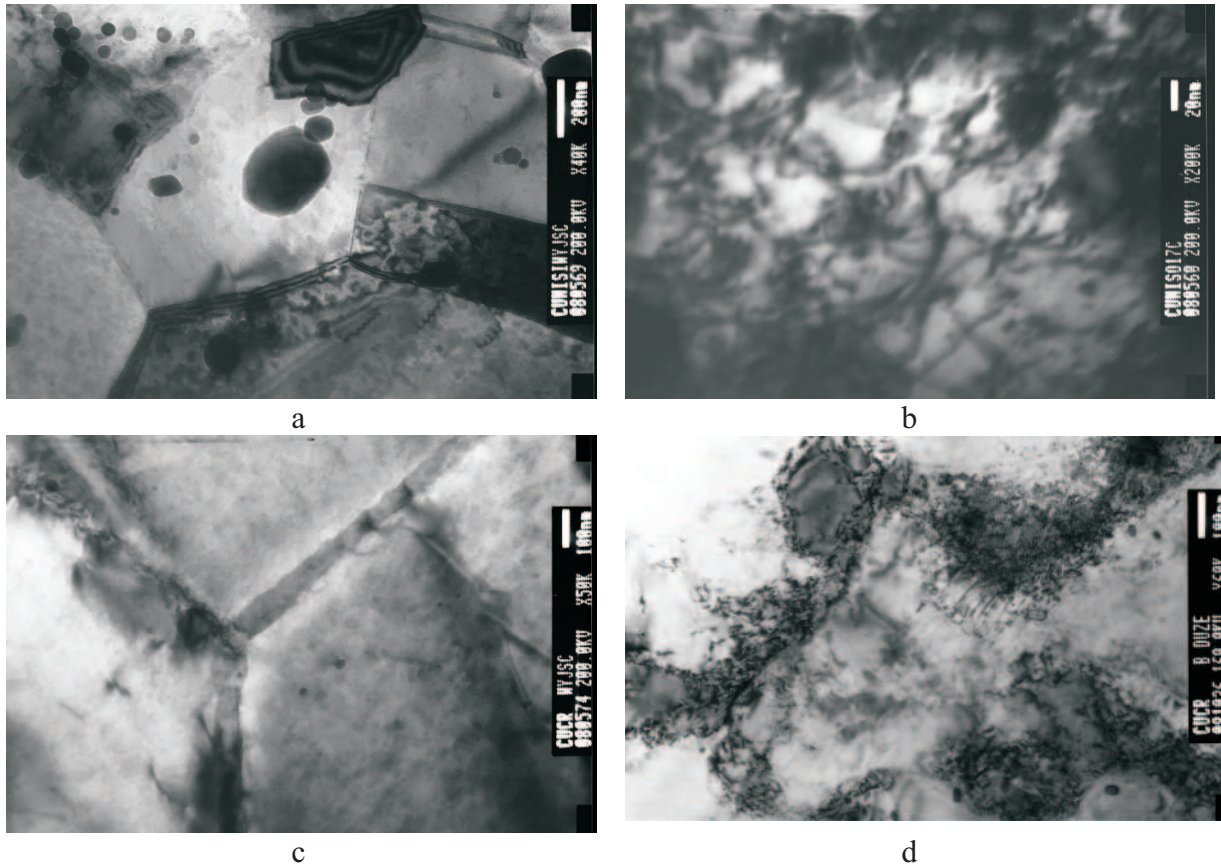
Fig. 6. Microstructure of CuNiSi alloy strips: as annealed (a), after 34 passes of deformation (b); and CuCr alloy strips: as annealed (c), after 34 passes of deformation (d); TEM
