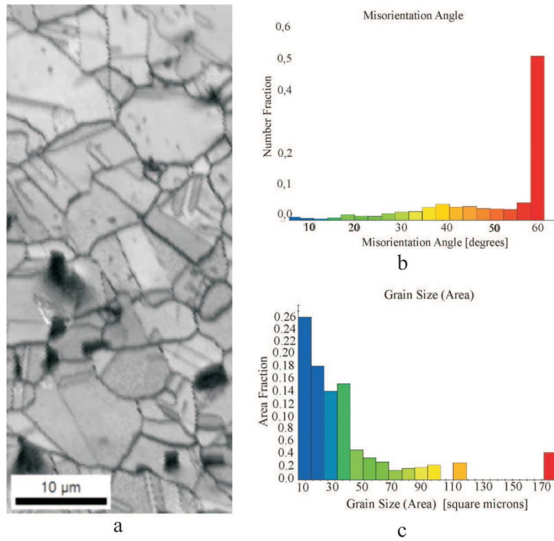
Fig. 4. Microstructure of CuCr alloy strip as annealed (a), with grain boundaries disorientation (b) and grain size distribution (c), SEM with EBSD
