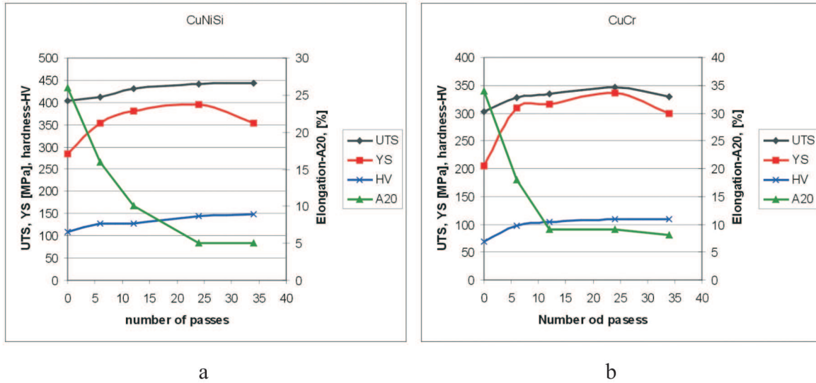
Fig. 7. Changes of mechanical properties of CuNiSi (a) and CuCr (b) strip during CRCS processing
