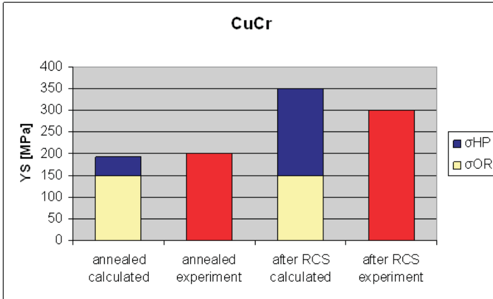
Fig. 8. Comparison of yield strength value calculated and obtained in experiment for CuCr alloy
