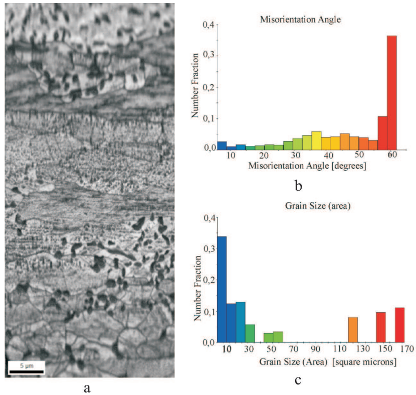
Fig. 2. Microstructure of CuNiSi alloy strip as annealed (a), with grain boundaries disorientation (b) and grain size distribution (c), SEM with EBSD
