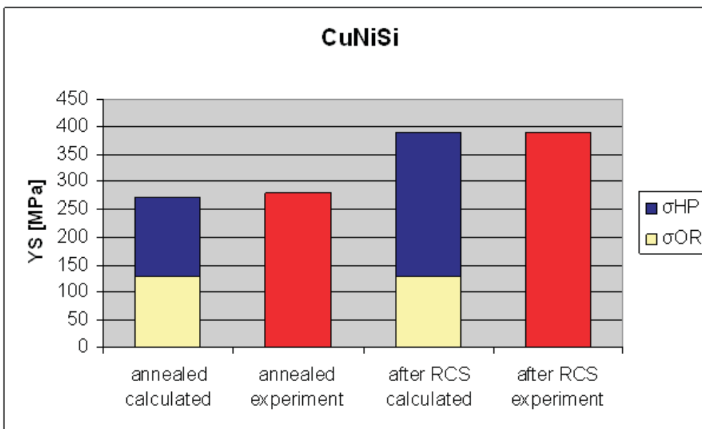
Fig. 9. Comparison of yield strength value calculated and obtained in experiment for CuNiSi alloy
