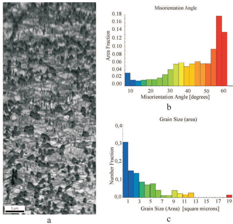
Fig. 3. Microstructure of CuNiSi alloy strip after 34 passes of deformation (a), with grain boundaries disorientation (b) and grain size distribution (c), SEM with EBSD
