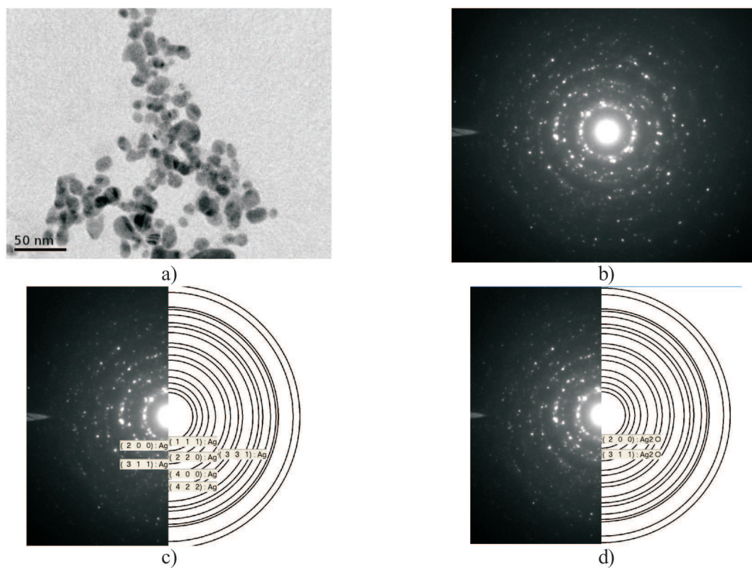
Fig. 5. TEM analysis of silver nanoparticles acquired during chronoamperometric polarization in alcoholic solutions of 0,001M \text{LiClO}_4 ( n\text{-C}_3\text{H}_7\text{OH} , E=1\text{V} , t=3\text{h} , T=298\text{K} ): a) morphology, b) electron diffraction, c) cubic silver match, d) \text{Ag}_2\text{O} match
