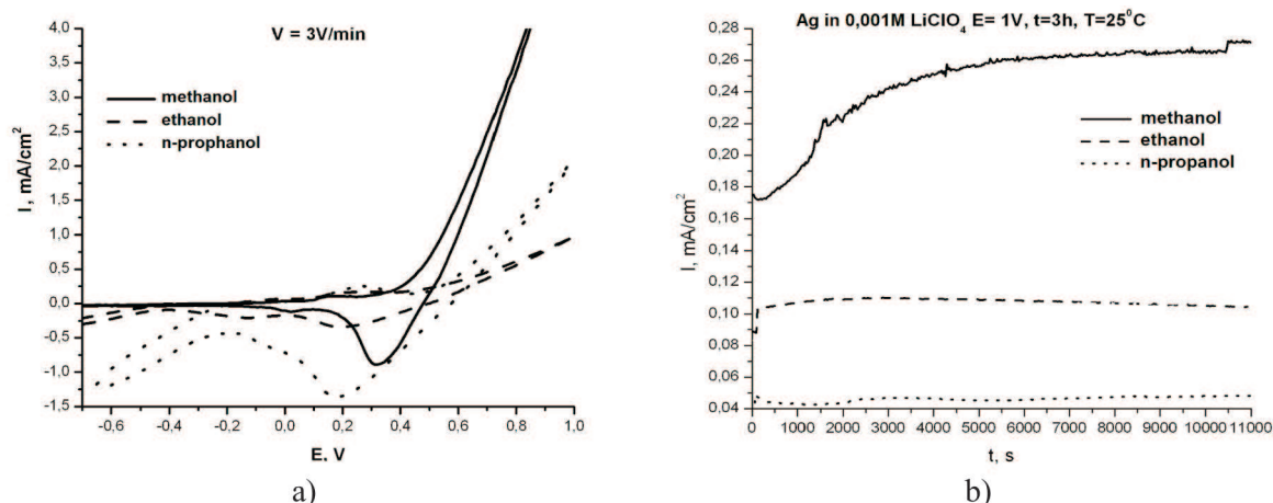
Fig. 1. Polarization curves for silver in various solvents, a) LSV curves, b) chronoamperometric curves
