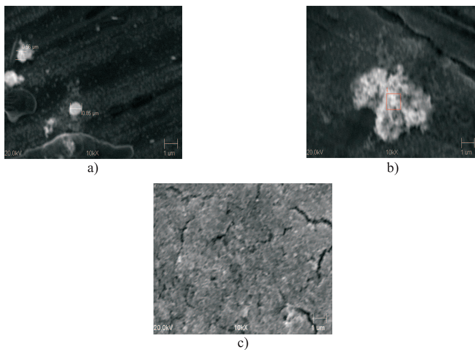
Fig. 2. SEM analysis of silver nanoparticles acquired during chronoamperometric polarization in alcoholic solutions of \text{LiClO}_4 (0,001M): a) \text{CH}_3\text{OH} ; b) \text{C}_2\text{H}_5\text{OH} ; c) \text{n-C}_3\text{H}_7\text{OH}
