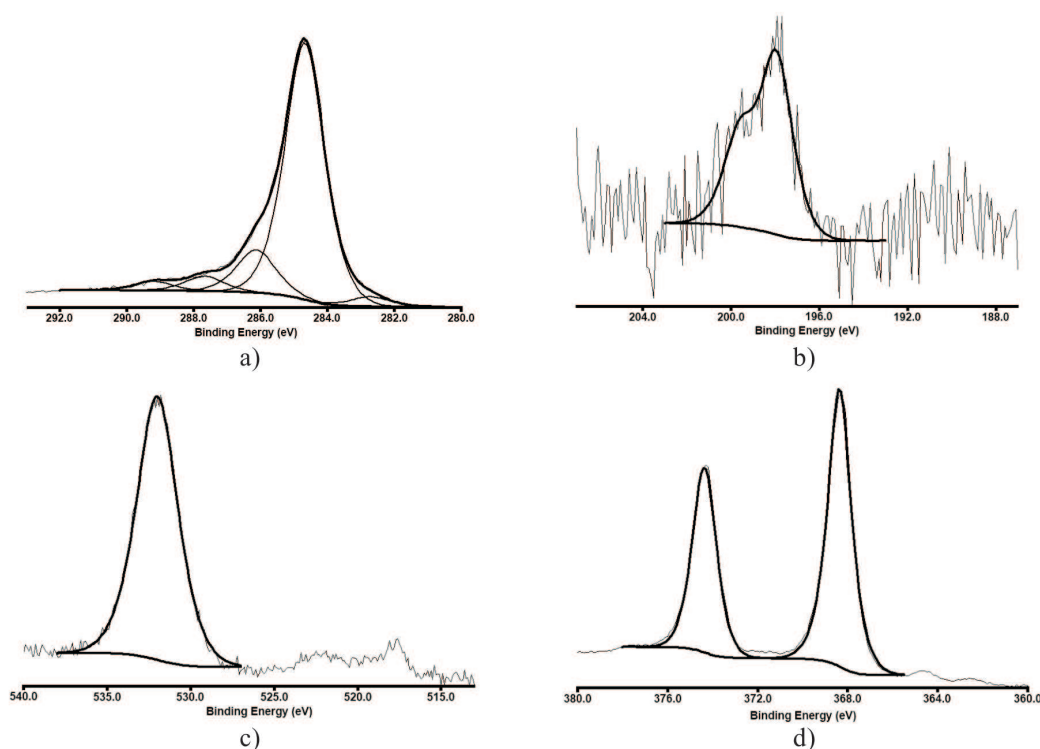
Fig. 6. XPS spectra of silver nanoparticles acquired in 0.001M LiClO 4 – C 2 H 5 OH solution, (E=1V), t=3h, T = 298 K in the bands: a) C 1s, b) Cl 2p, c) O 1s, d) Ag 3d
