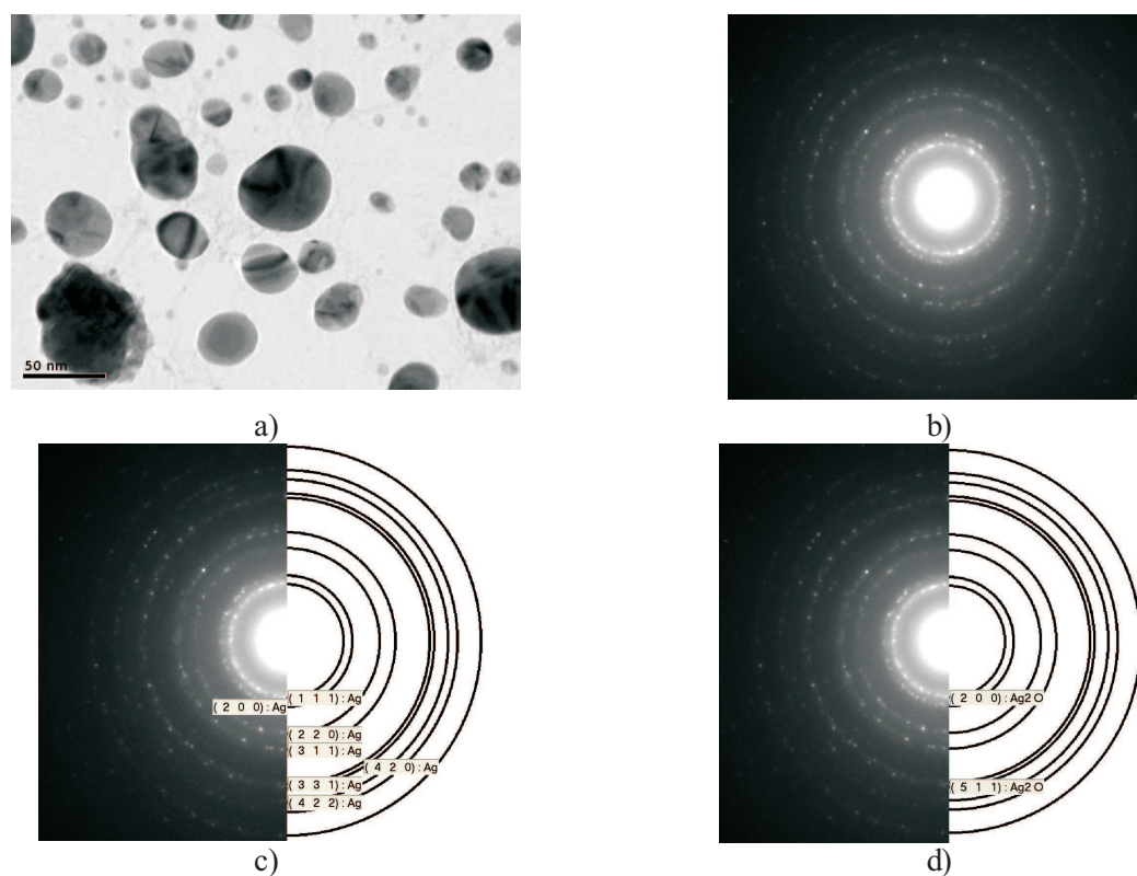
Fig. 3. TEM analysis of silver nanoparticles acquired during chronoamperometric polarization in alcoholic solutions of 0,001M \text{LiClO}_4 ( \text{CH}_3\text{OH} , E=1\text{V} , t=3\text{h} , T=298\text{K} ): a) morphology, b) electron diffraction, c) cubic silver match, d) \text{Ag}_2\text{O} match
