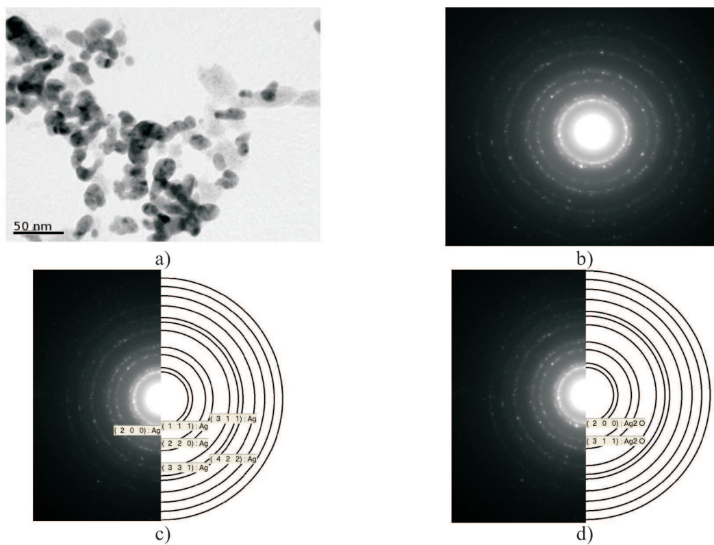
Fig. 4. TEM analysis of silver nanoparticles acquired during chronoamperometric polarization in alcoholic solutions of 0,001M \text{LiClO}_4 ( \text{C}_2\text{H}_5\text{OH} , E=1\text{V} , t=3\text{h} , T=298\text{K} ): a) morphology, b) electron diffraction, c) cubic silver match, d) \text{Ag}_2\text{O} match
