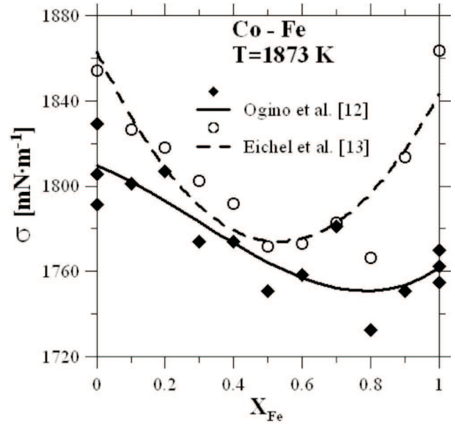
Fig. 7. Surface tension of Fe-Co alloys at 1873K
