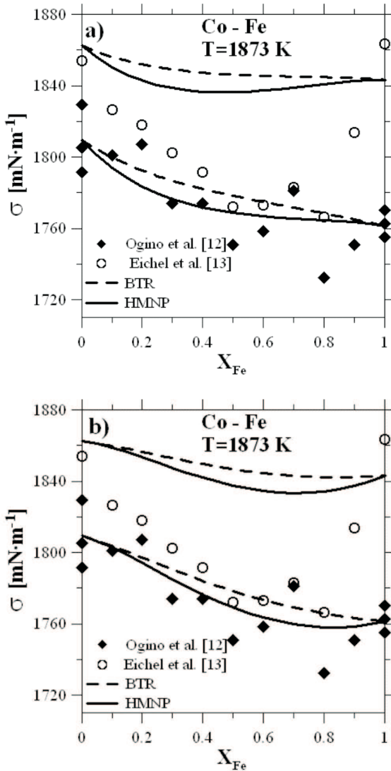
Fig. 9. Calculated and experimental surface tension [12, 13] at 1873K. G^{ex} used in surface tension modeling was calculated from the data of a) Belton and Predel [16,18] and b) Batalin and Predel [17,18], respectively
