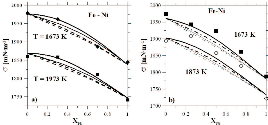
Fig. 5. Values of the surface tension in Fe-Ni system: a) calculated [7] and b) experimental [8]
