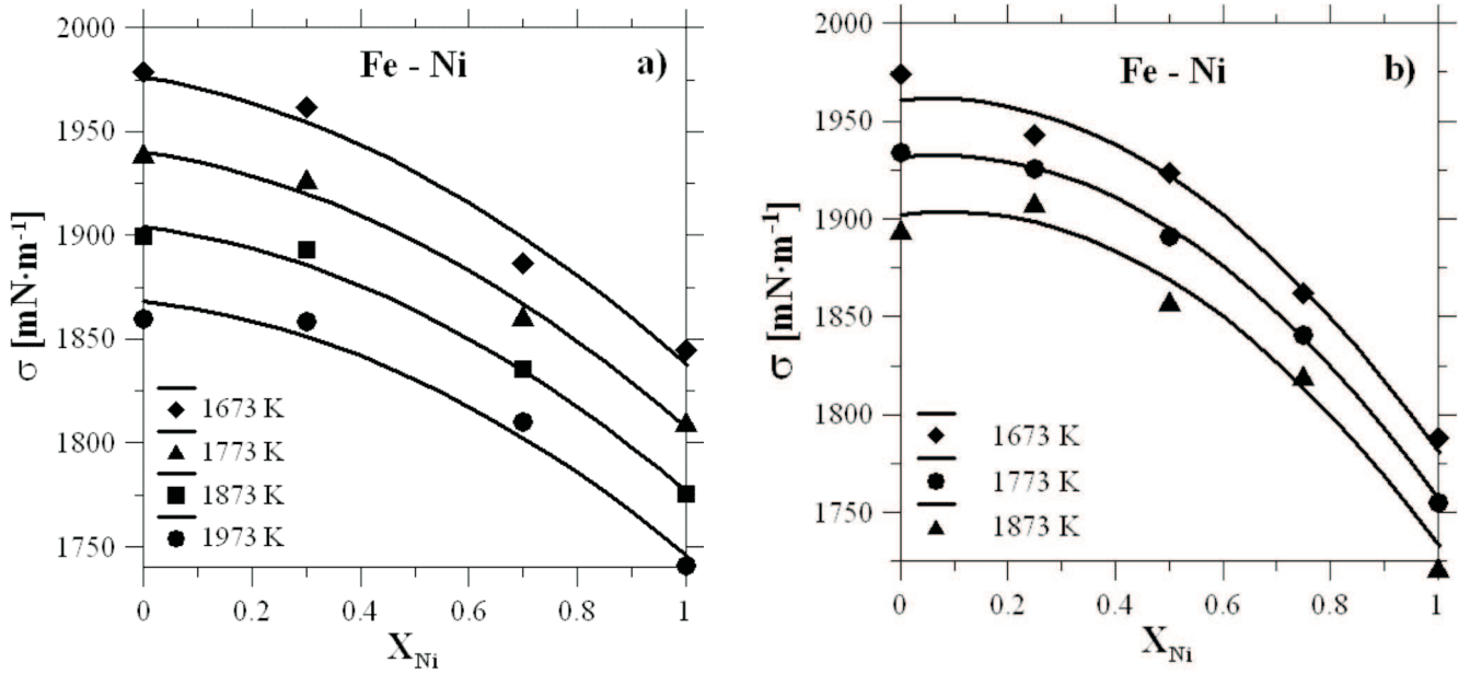
Fig. 4. Surface tension dependence on composition in Fe-Ni system. Data of a) Lee et al. [7], b) Brillo and Egly [8], respectively
