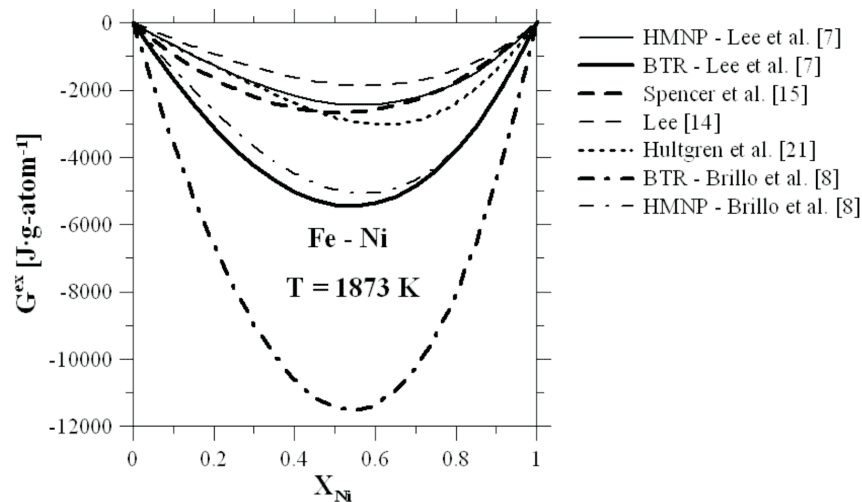
Fig. 6. Calculated and experimental [14, 15, 21] thermodynamic properties of the Fe-Ni system at 1873K
