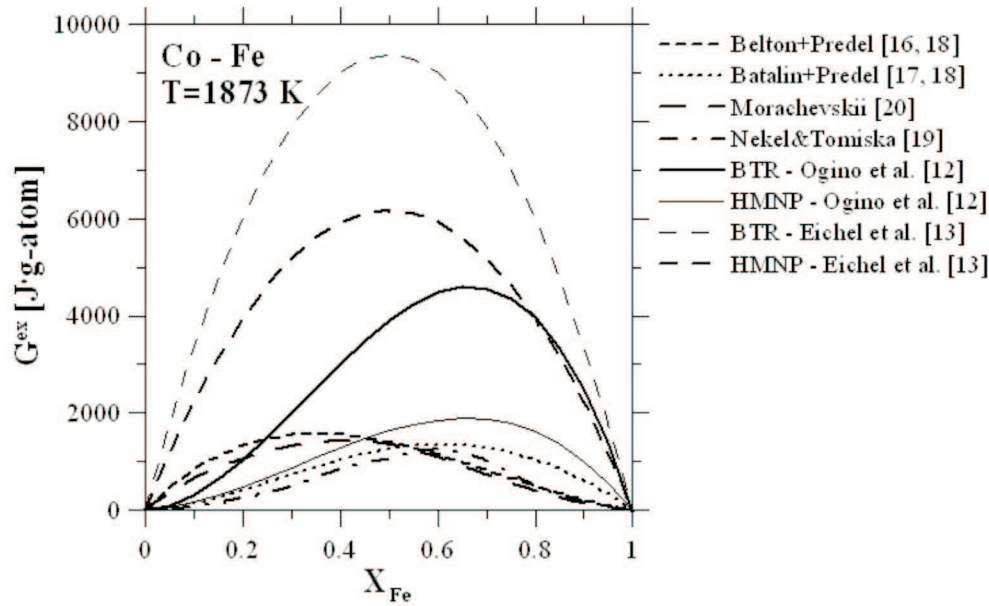
Fig. 10. Excess Gibbs free energy of the Fe-Co system calculated from the models and obtained from the experiments [16-20]
