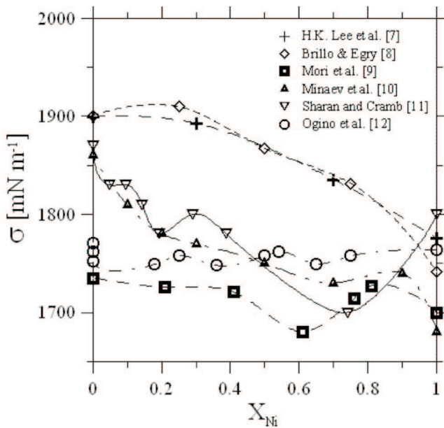
Fig. 3. Surface tension dependence on composition in Fe-Ni system. Data of [7,8,12] at 1873K and data of [9-11] at 1823K. Lines are used to suggest the trends only
