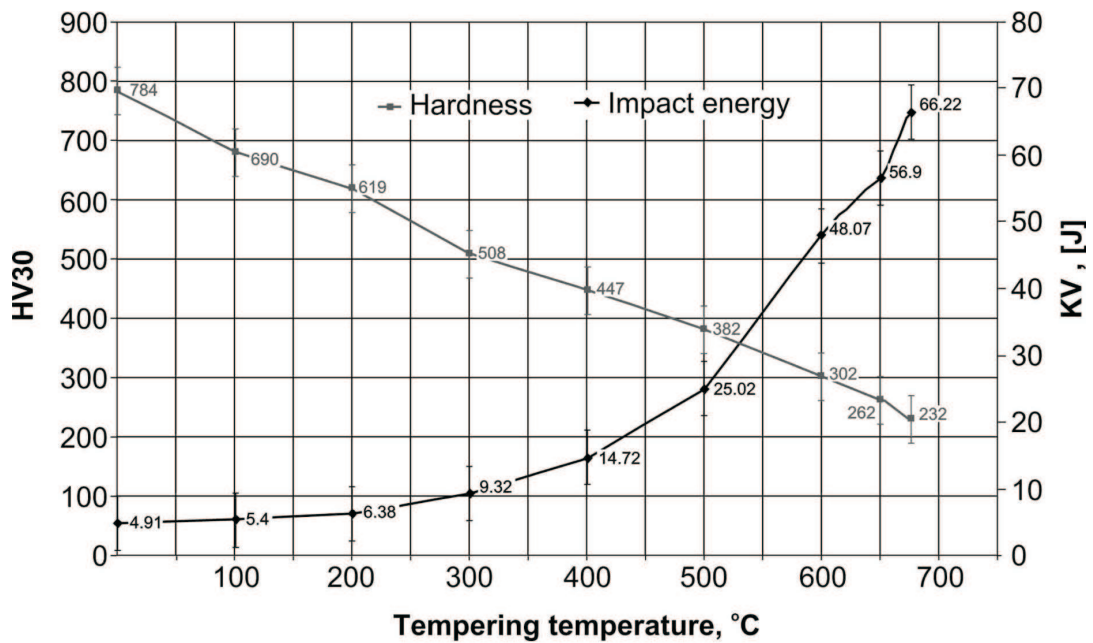
Fig. 4. Influence of the tempering temperature on impact energy (KV) and hardness (HV30) of the 56NiCrMo7 steel samples, quenched in oil from a temperature of 800^\circ\text{C}
