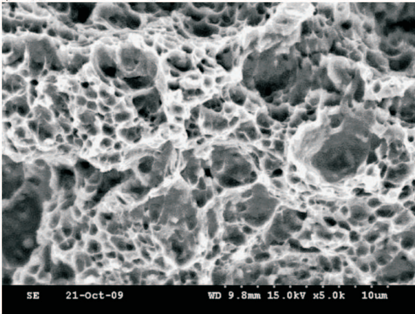
Fig. 5. Photographs of the 56NiCrMo7 steel sample fractures: quenched in oil from 800^\circ\text{C} (Fig. 5 a) and then tempered for 2 hours at temperatures: 100, 200, 300, 400, 500, 600, 650 and 675^\circ\text{C} (Fig. 5 b÷i)
