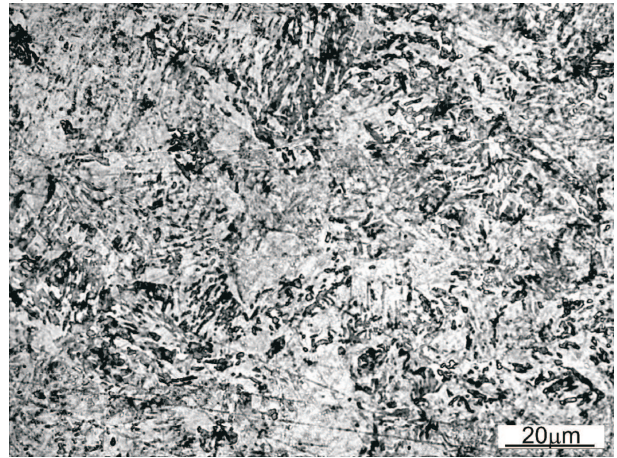
Fig. 3. Photographs of microstructures of the selected 56NiCrMo7 steel samples tempered in the temperature range 100\div 650^\circ\text{C} , previously quenched in oil from 800^\circ\text{C}
