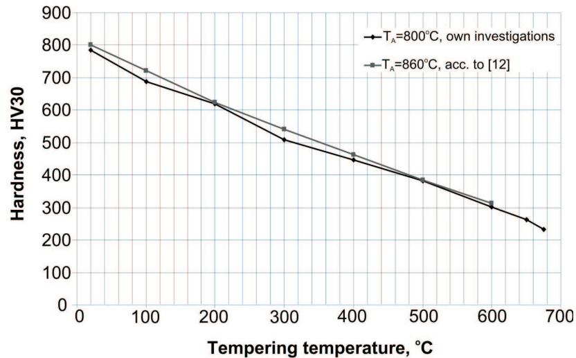
Fig. 2. Influence of the tempering temperature on hardness (HV30) of the 56NiCrMo7 steel samples quenched in oil from 800°C (own investigations) and from 860°C (acc. to [12])
