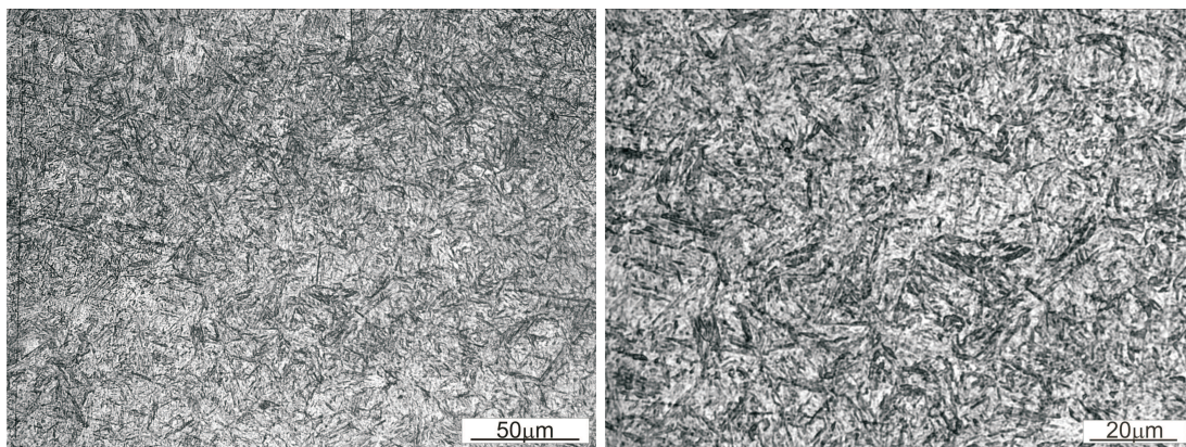
Fig. 1. Photographs of the microstructure of the 56NiCrMo7 steel sample quenched in oil from 800°C
