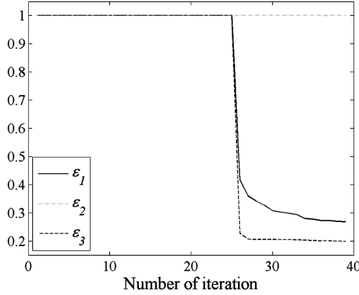
Figure 7. The coefficients of energy weighting matrix versus iterations.
