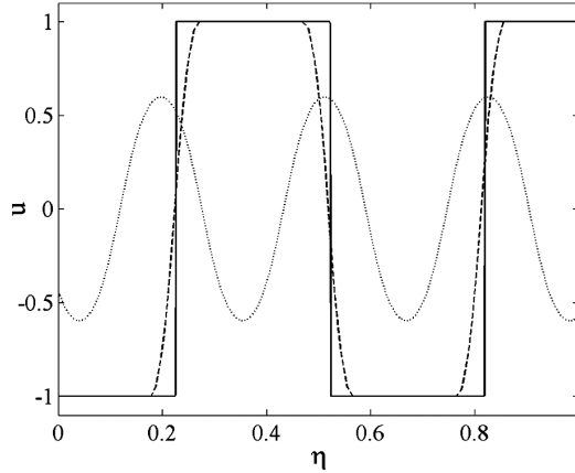
Figure 4. Optimal input controls for different final times (solid line: t_f^{(41)} , dashed line: t_f^{(21)} , dotted line: t_f^{(0)} ).
