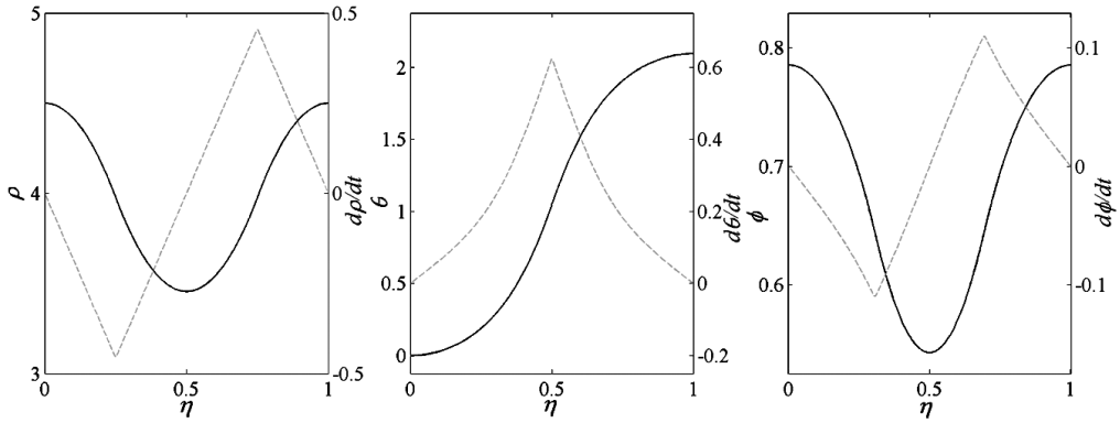
Figure 5. Time optimal states versus non-dimensional time. (dashed line refers to the right y-axis, solid line refers to the left y-axis).
