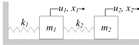
Figure 8. Schematic image of double spring-mass system.
