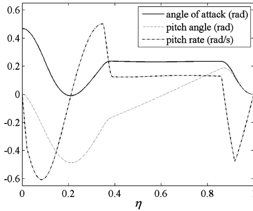
Figure 11. Time optimal states versus non-dimensional time.
