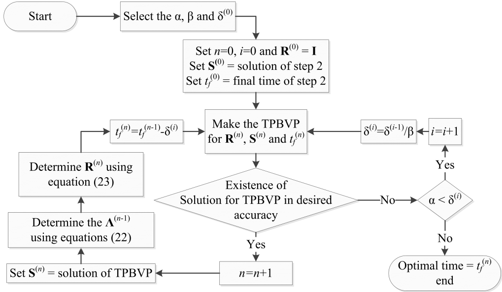
Figure 1. Flowchart of minimum time calculation (last phase).
