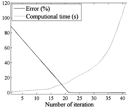
Figure 2. Percentage of error and computational time versus iterations.
