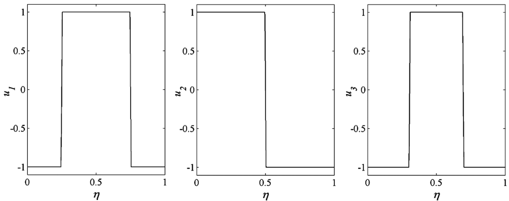
Figure 6. Time optimal controls versus non-dimensional time.
