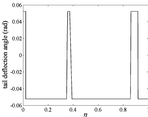
Figure 12. Time optimal control versus non-dimensional time.
