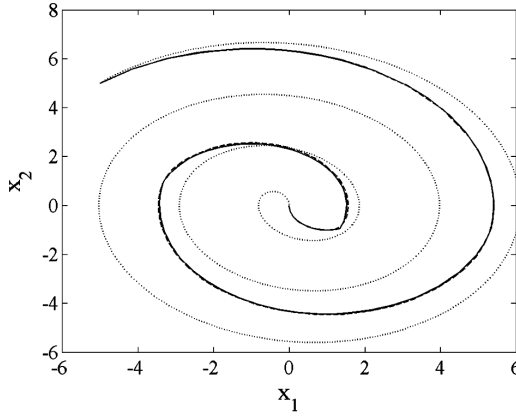
Figure 3. Optimal phase planes for different final times (solid line: t_f^{(41)} , dashed line: t_f^{(21)} , dotted line: t_f^{(0)} ).
