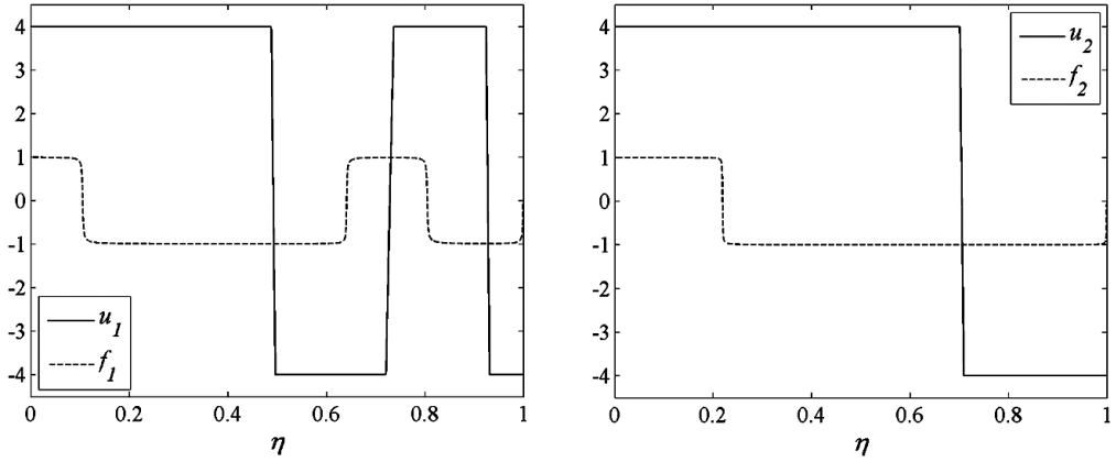
Figure 10. Time optimal controls and frictional forces versus non-dimensional time.
