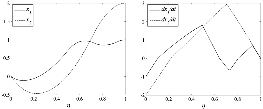
Figure 9. Time optimal states versus non-dimensional time.
